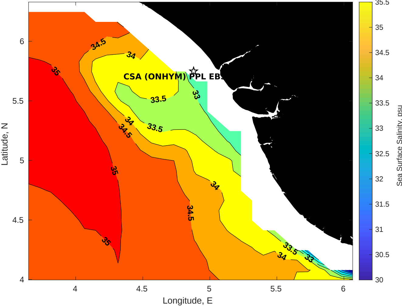
Surface Salinity for CSA (ONHYM) PPL EBS - Nigeria at 01-May-2025 00:00:00
