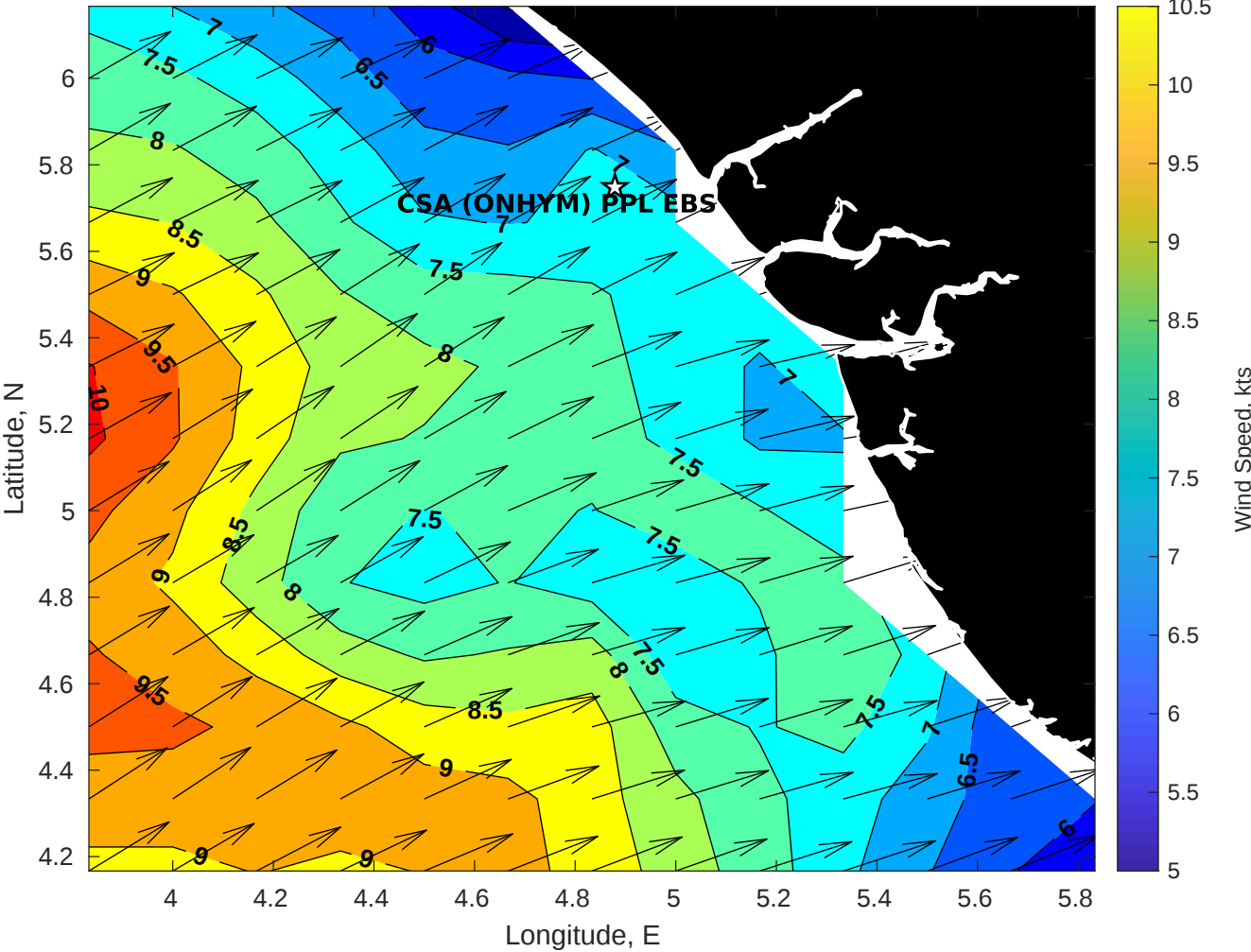
Winds (kts) for CSA (ONHYM) PPL EBS - Nigeria at 02-May-2025 09:00:00
