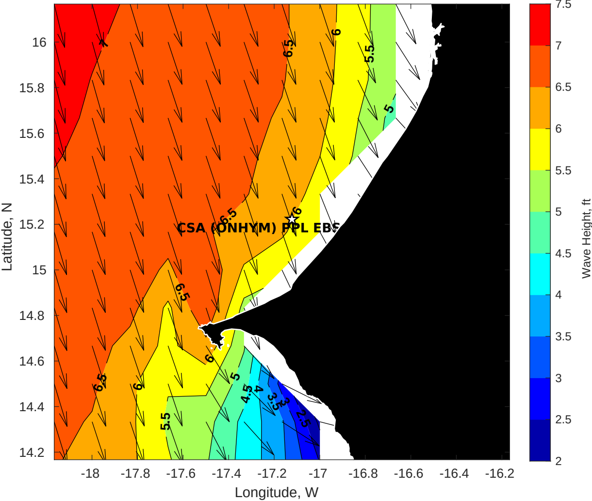
Wave Height (ft) for CSA (ONHYM) PPL EBS - Senegal at 02-May-2025 09:00:00
