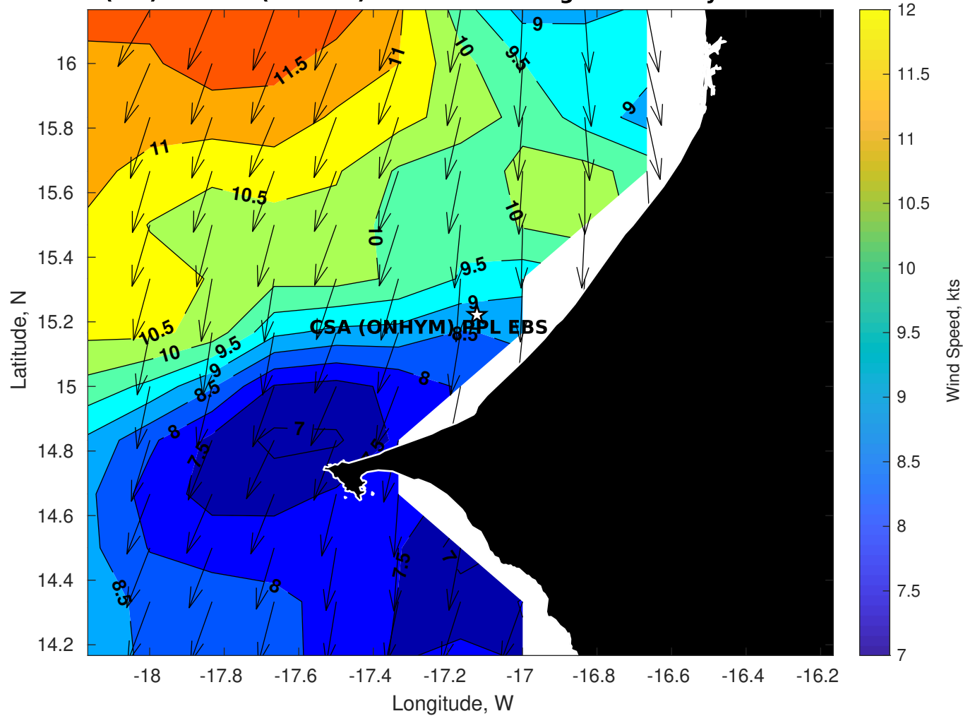
Winds (kts) for CSA (ONHYM) PPL EBS - Senegal at 02-May-2025 09:00:00
