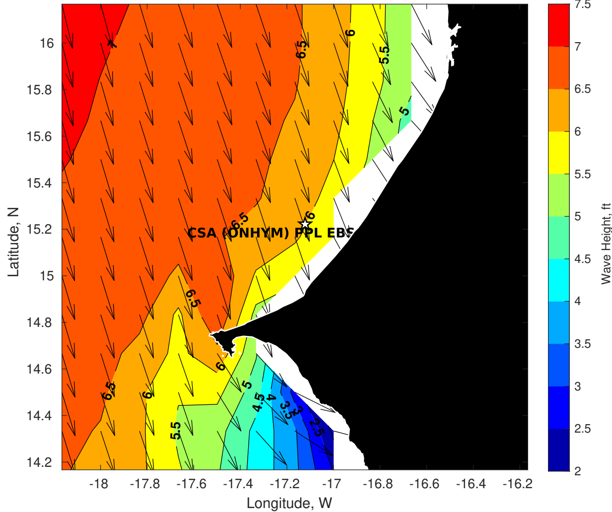
Wave Height (ft) for CSA (ONHYM) PPL EBS - Senegal at 02-May-2025 09:00:00
