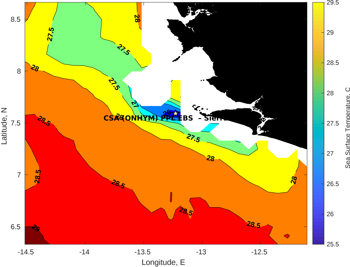
SST for CSA (ONHYM) PPL EBS - Sierra Leone at 01-May-2025 00:00:00
