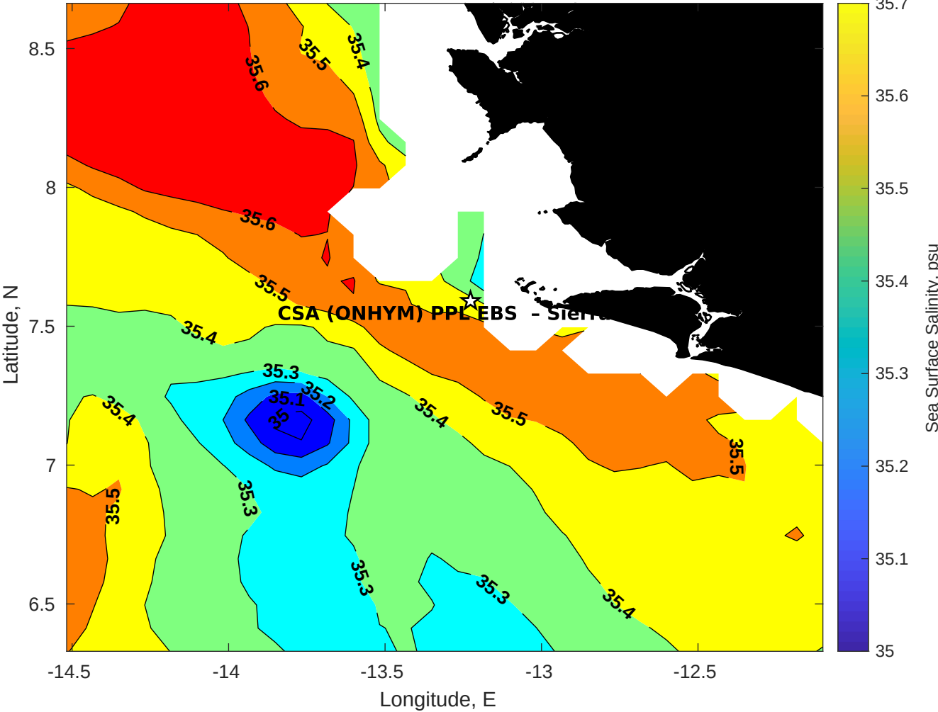
Surface Salinity for CSA (ONHYM) PPL EBS - Sierra Leone at 01-May-2025 00:00:00
