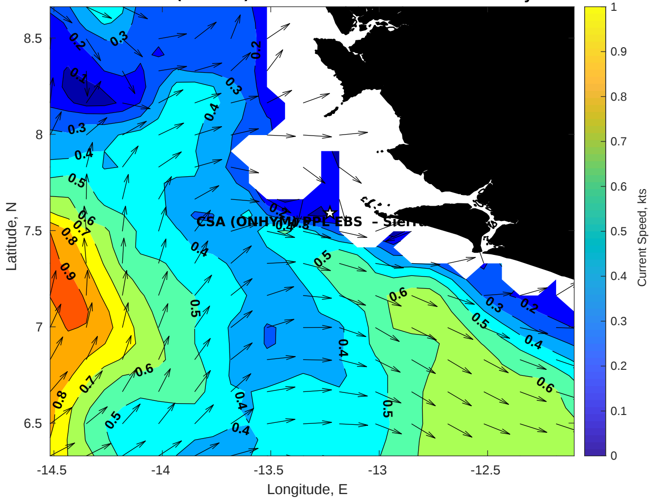
Surface Currents for CSA (ONHYM) PPL EBS - Sierra Leone at 01-May-2025 00:00:00
