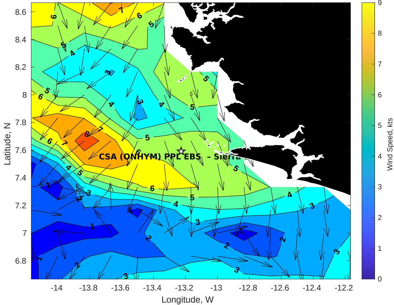
Winds (kts) for CSA (ONHYM) PPL EBS - Sierra Leone at 02-May-2025 09:00:00
