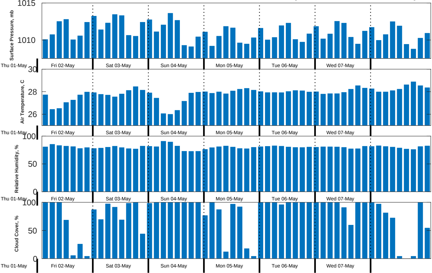
Met Forecast for CSA (ONHYM) PPL EBS - Sierra Leone from 02-May-2025 00:00:00 to 09-May-2025 00:00:00
