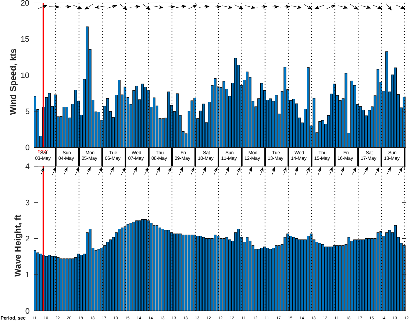
Wind & Wave Forecast for CSA (ONHYM) PPL EBS - Sierra Leone from 02-May-2025 01:00:00 to 18-May-2025 01:00:00
