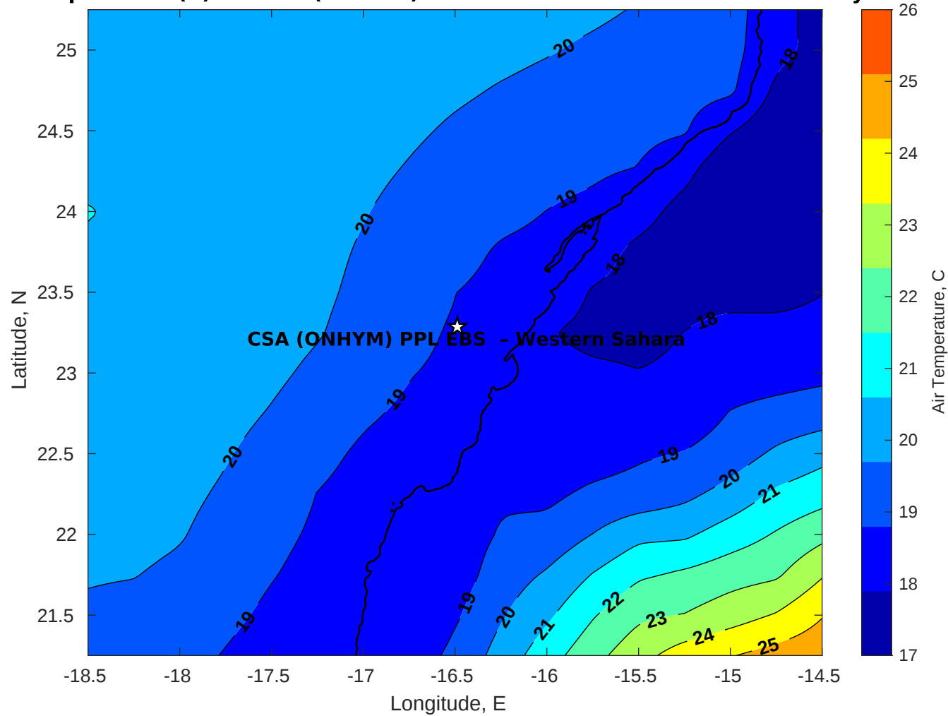
Air Temperature (C) for CSA (ONHYM) PPL EBS - Western Sahara at 02-May-2025
