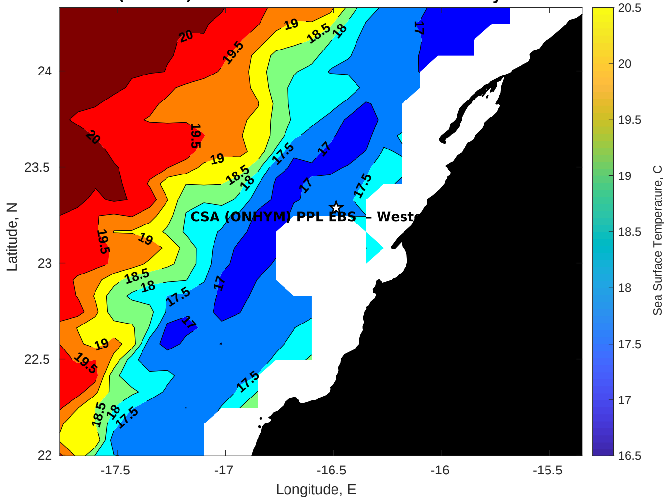
SST for CSA (ONHYM) PPL EBS - Western Sahara at 01-May-2025 00:00:00
