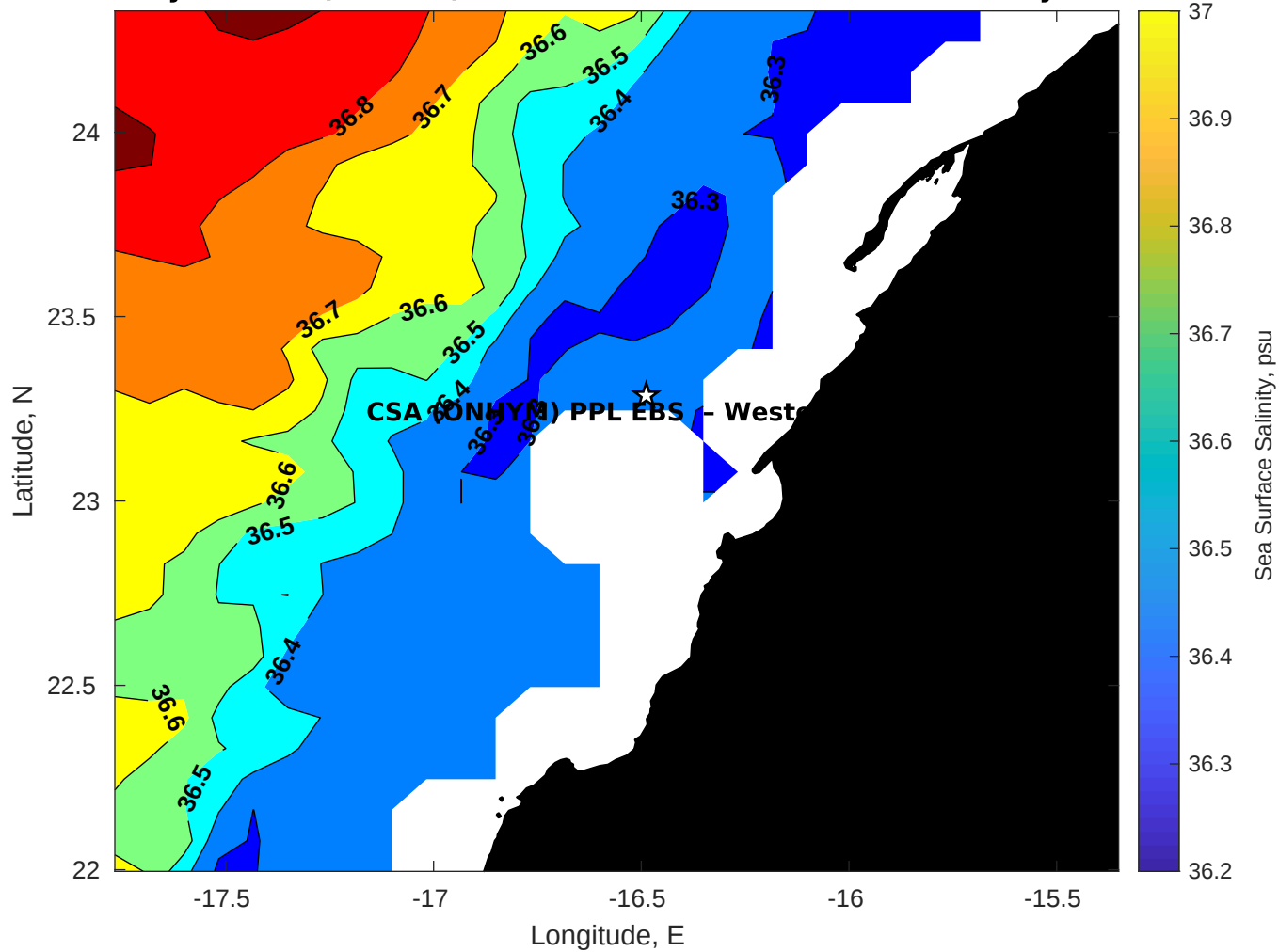
Surface Salinity for CSA (ONHYM) PPL EBS - Western Sahara at 01-May-2025 00:00:00
