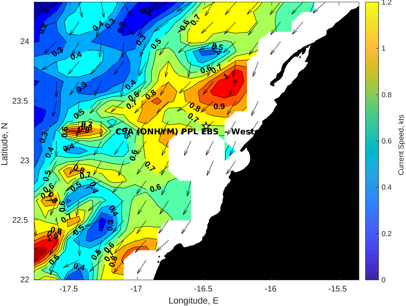
Surface Currents for CSA (ONHYM) PPL EBS - Western Sahara at 01-May-2025 00:00:00
