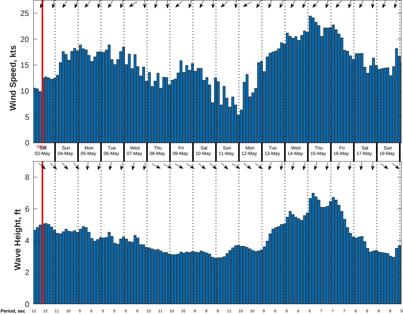
Wind & Wave Forecast for CSA (ONHYM) PPL EBS - Western Sahara from 02-May-2025 01:00:00 to 18-May-2025 01:00:00
