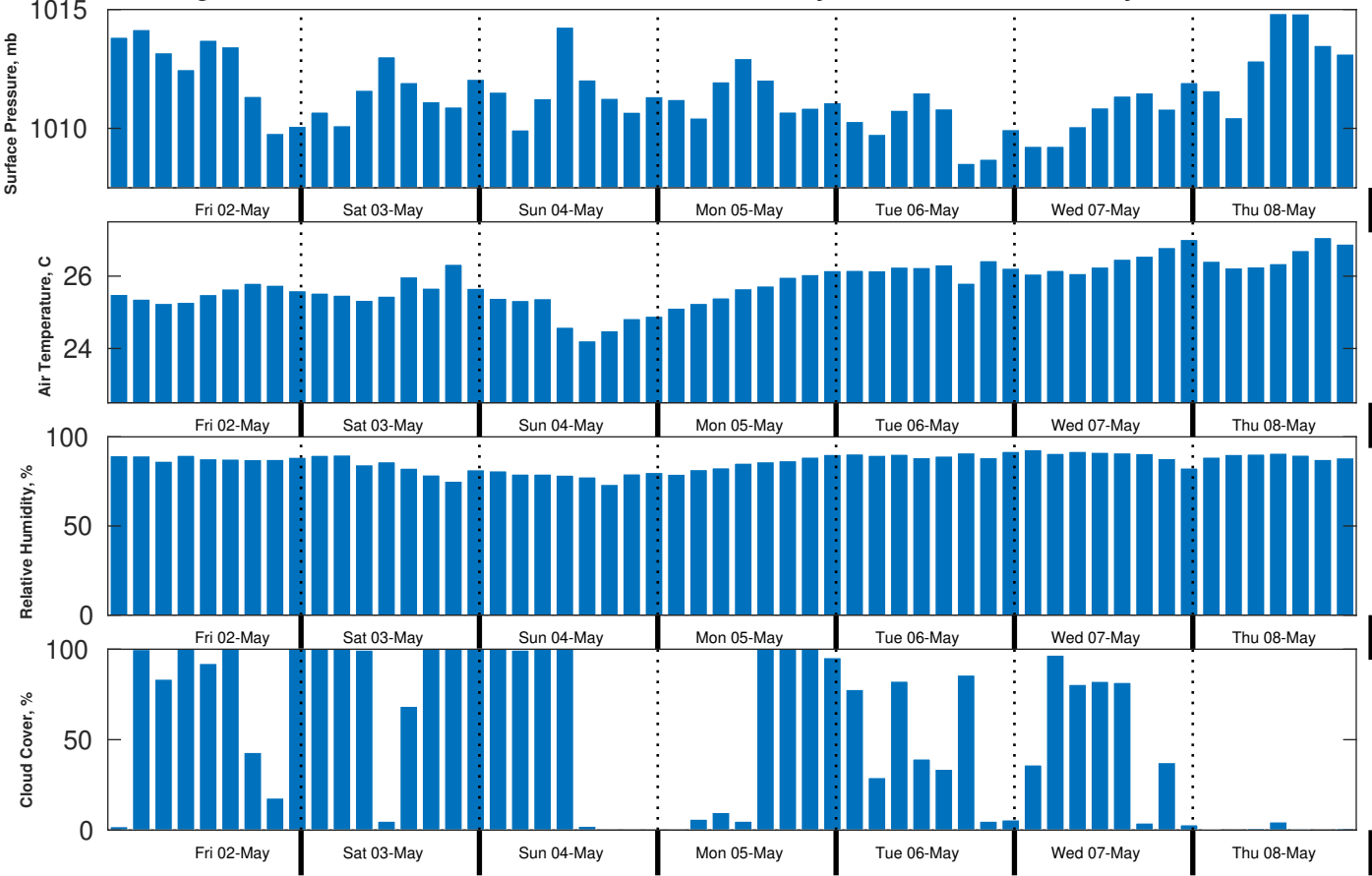
Met Forecast for CTI Enbridge Kaskida & Tiber PPL Geotechnical from 02-May-2025 00:00:00 to 09-May-2025 00:00:00
