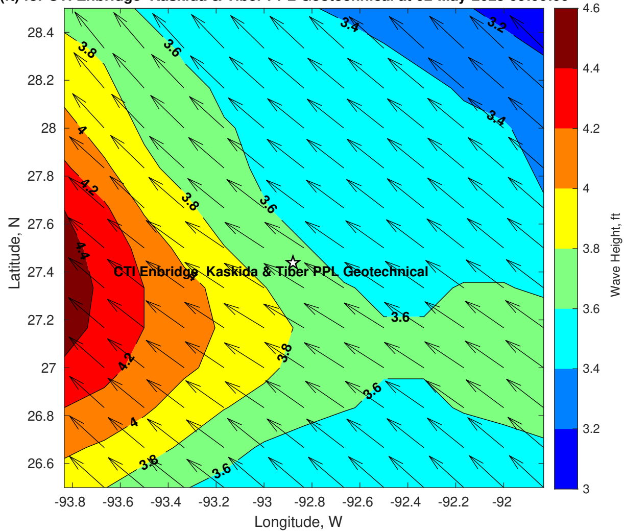
Wave Height (ft) for CTI Enbridge Kaskida & Tiber PPL Geotechnical at 02-May-2025 09:00:00
