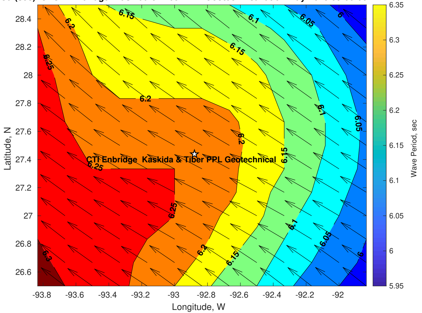
Wave Period (sec) for CTI Enbridge Kaskida & Tiber PPL Geotechnical at 02-May-2025 09:00:00
