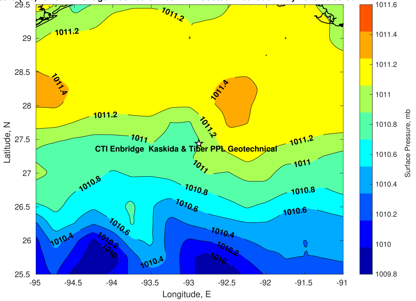
Surface Pressure (mb) for CTI Enbridge Kaskida & Tiber PPL Geotechnical at 04-May-2025 00:00:00
