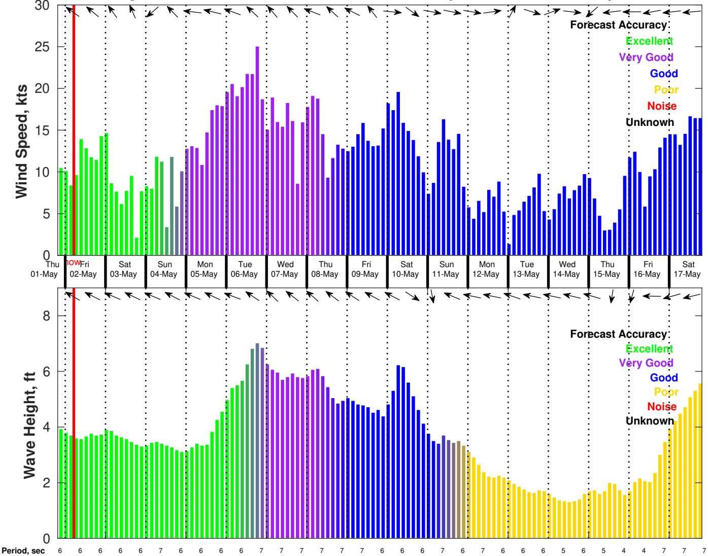
Wind & Wave Forecast for CTI Enbridge Kaskida & Tiber PPL Geotechnical from 01-May-2025 20:00:00 to 17-May-2025 20:00:00
