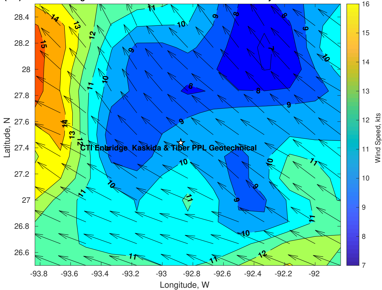
Winds (kts) for CTI Enbridge Kaskida & Tiber PPL Geotechnical at 02-May-2025 09:00:00
