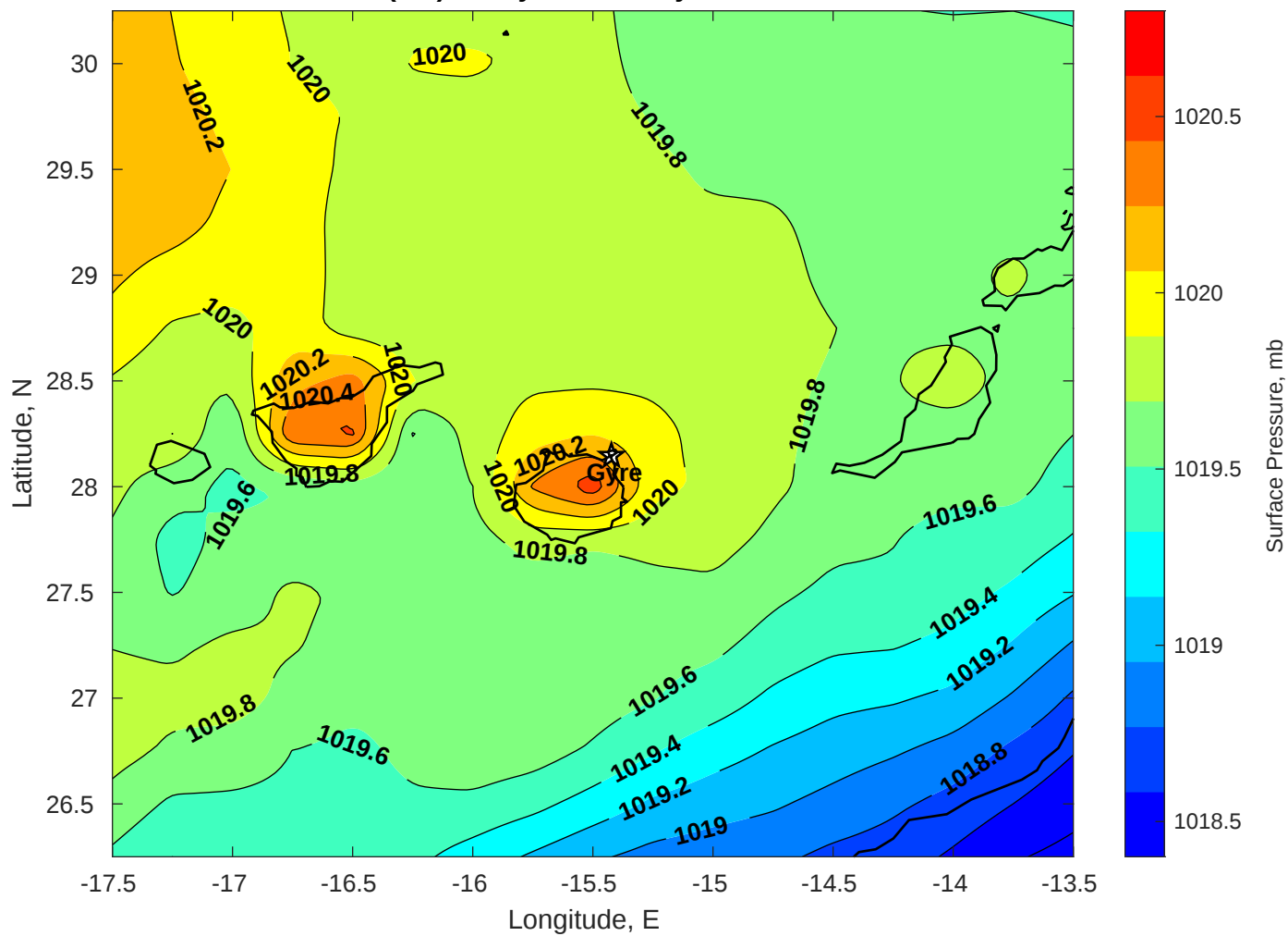
Surface Pressure (mb) for Gyre at 04-May-2025 00:00:00
