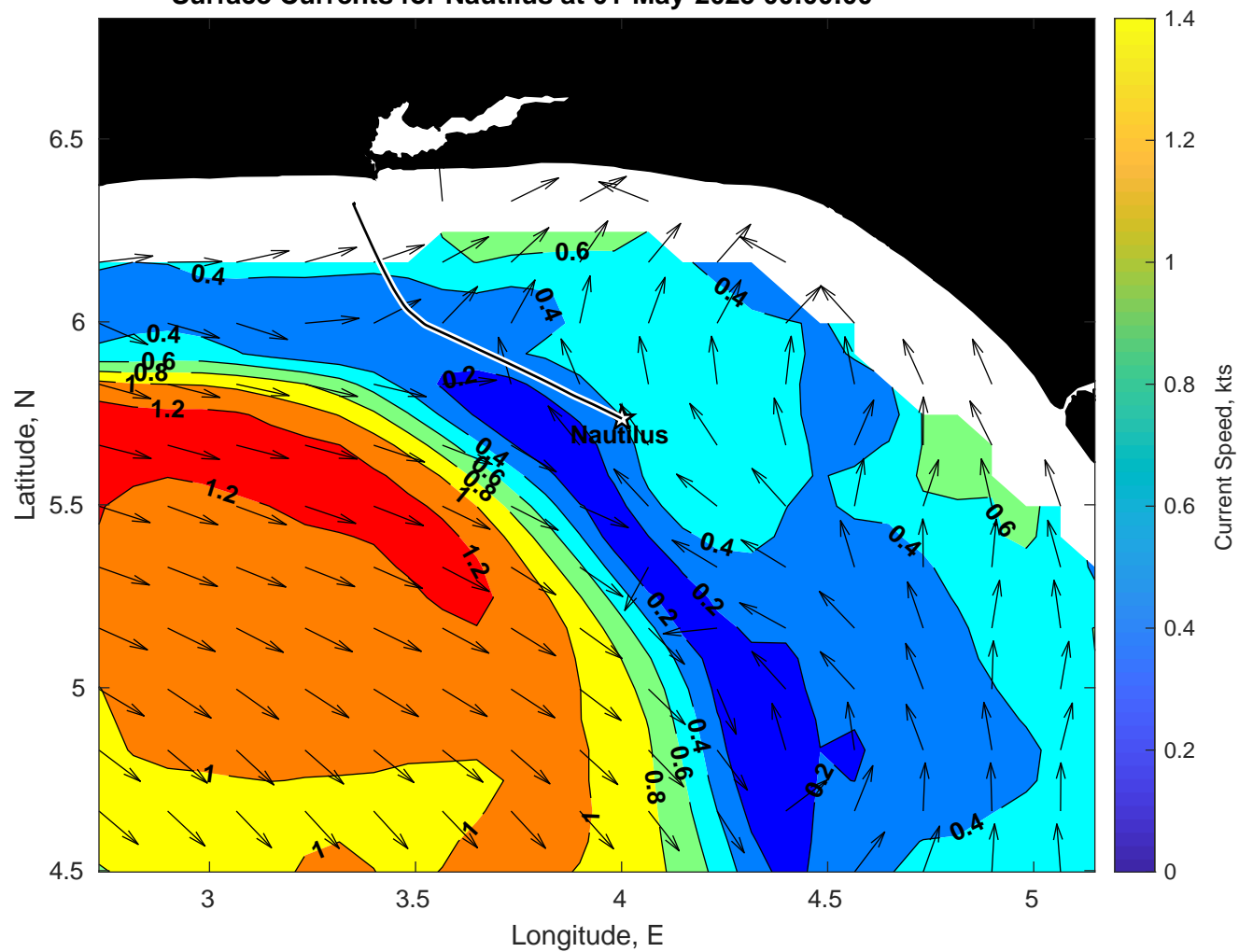
Surface Currents for Nautilus at 01-May-2025 00:00:00
