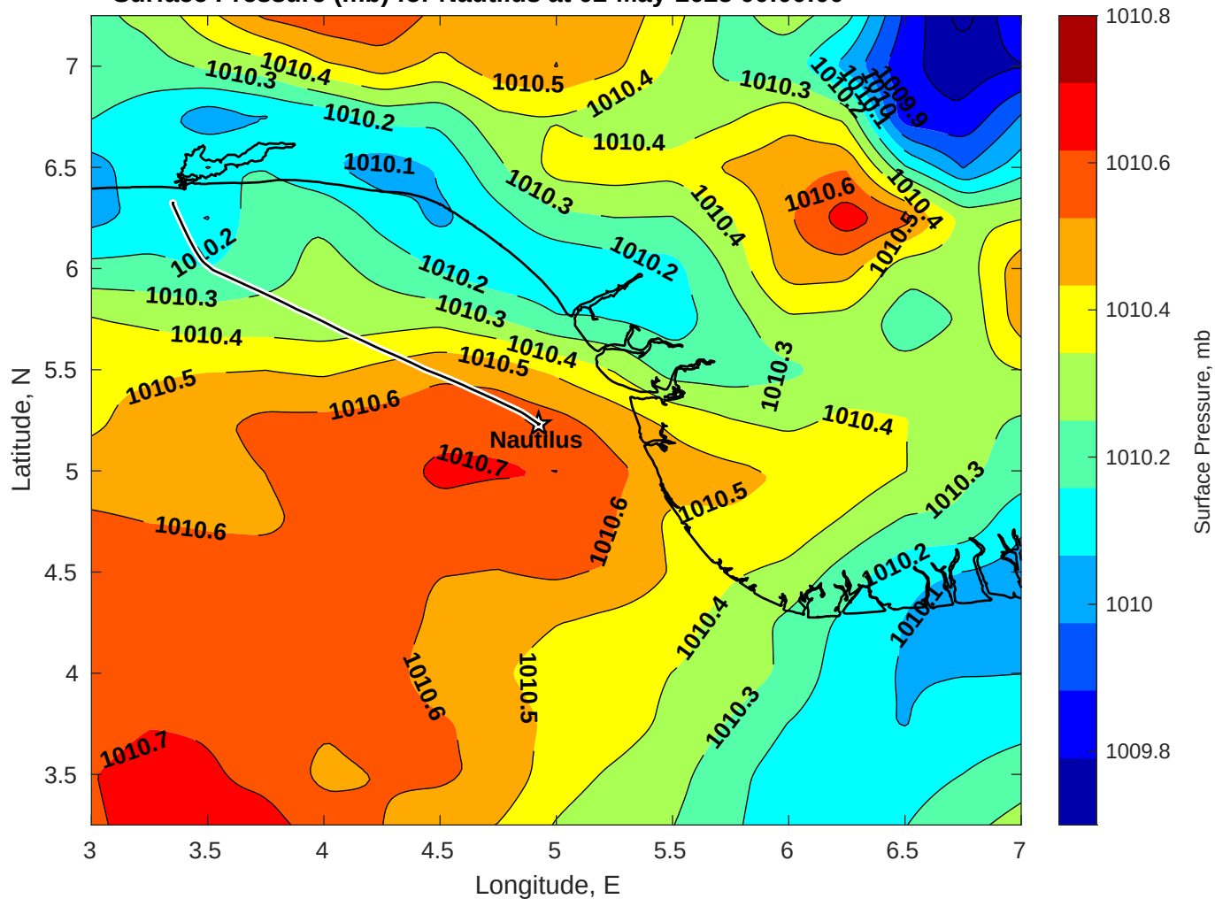
Surface Pressure (mb) for Nautilus at 02-May-2025 00:00:00
