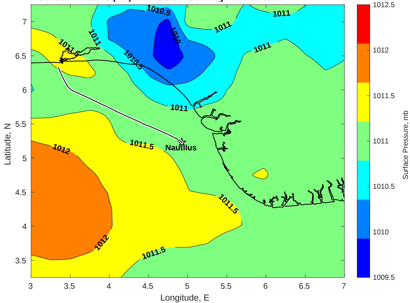
Surface Pressure (mb) for Nautilus at 04-May-2025 00:00:00
