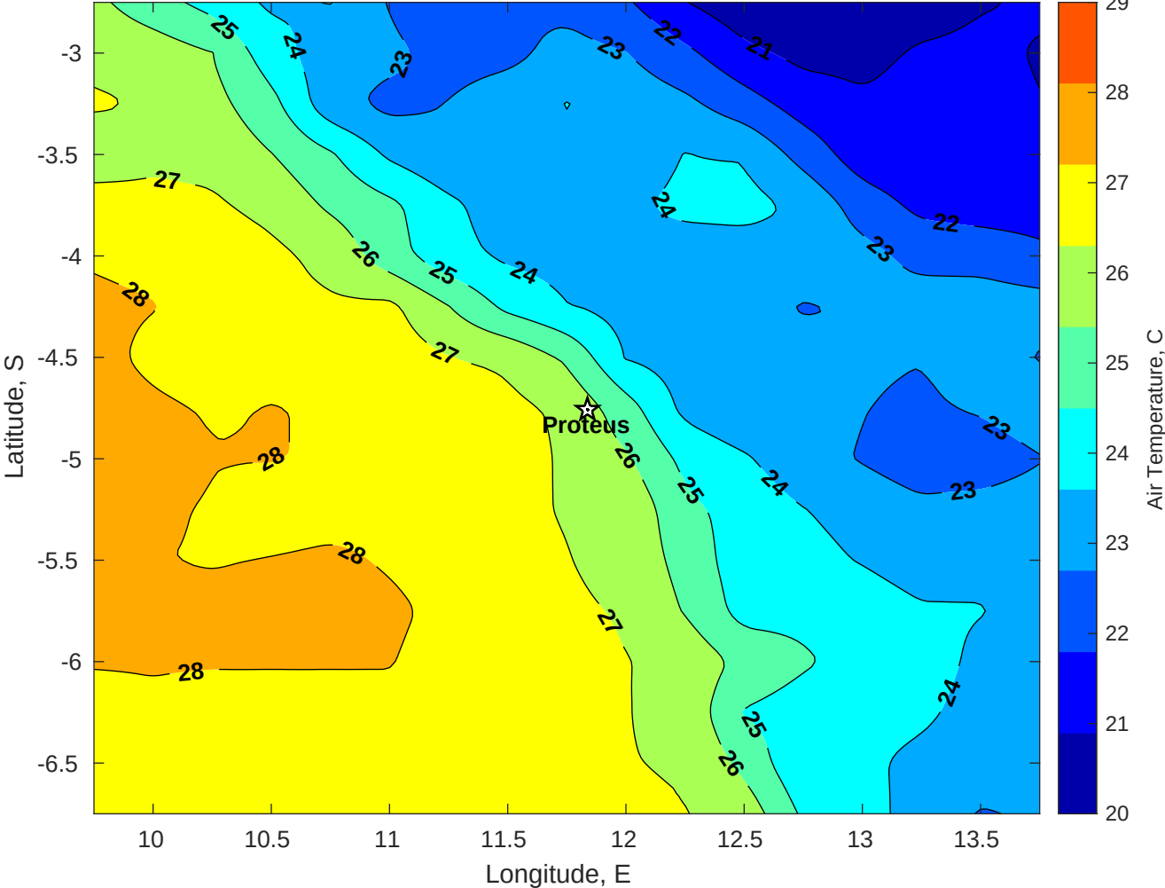
Air Temperature (C) for Proteus at 02-May-2025
