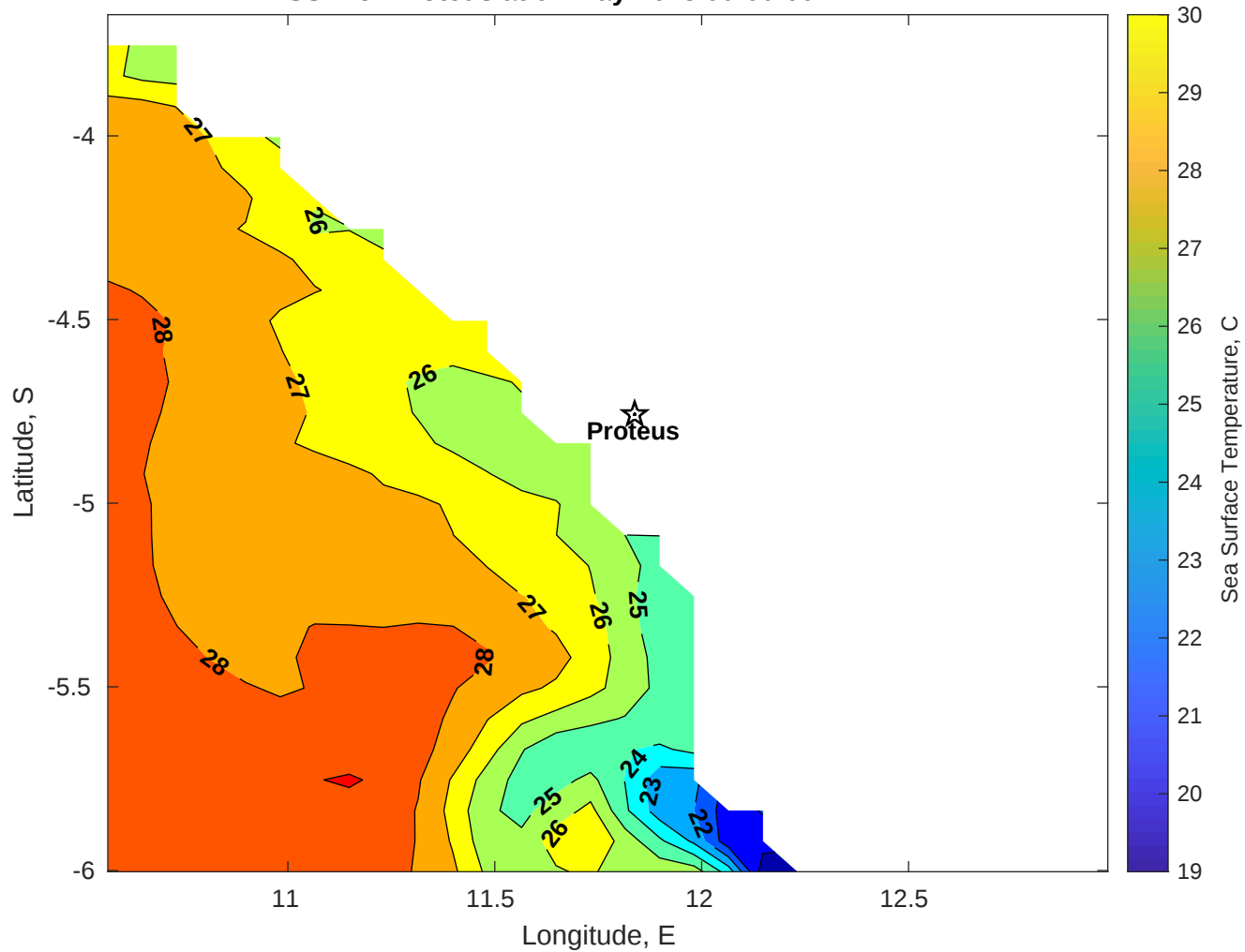
SST for Proteus at 01-May-2025 00:00:00
