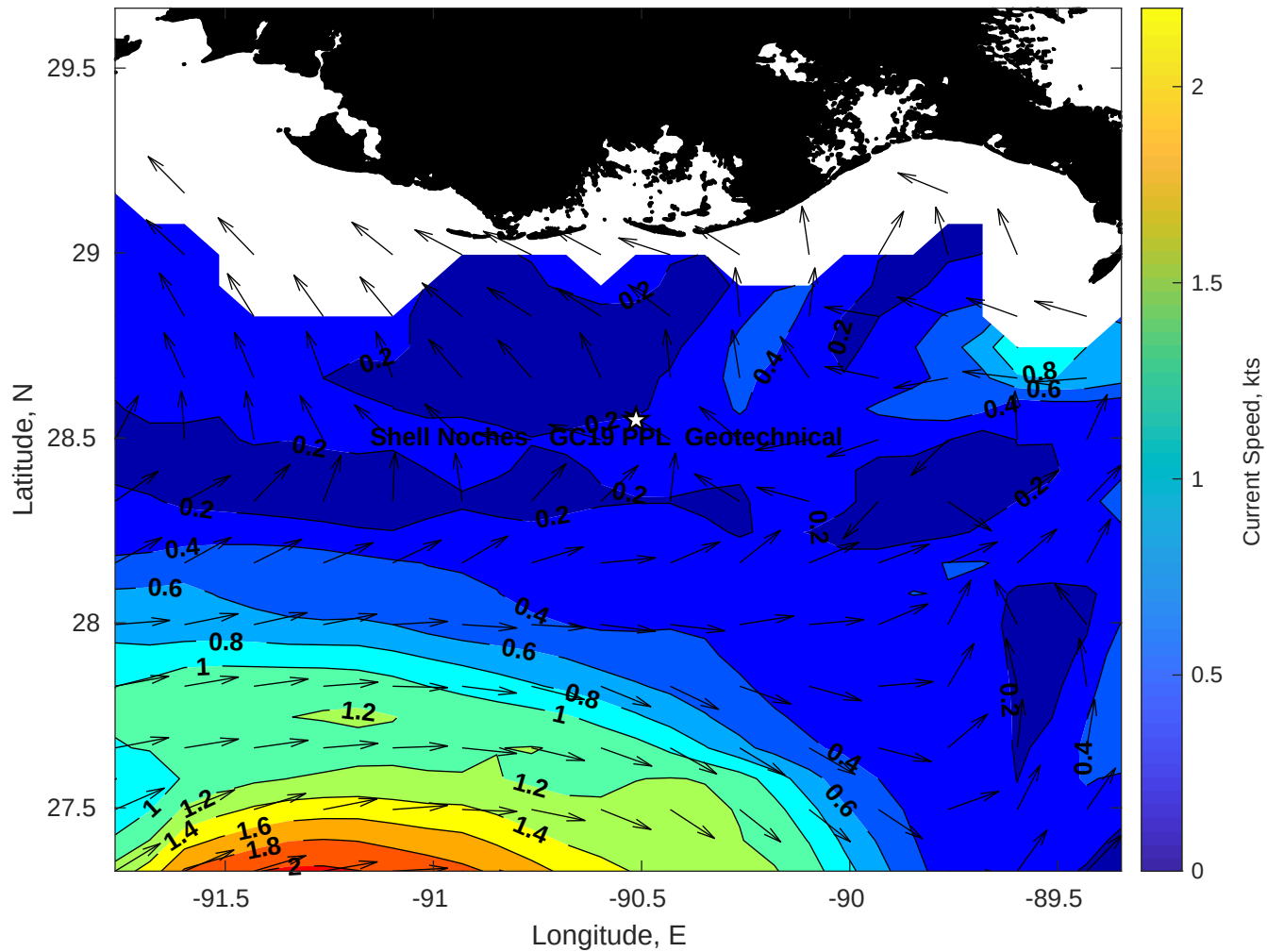
Surface Currents for Shell Noches GC19 PPL Geotechnical at 01-May-2025 00:00:00
