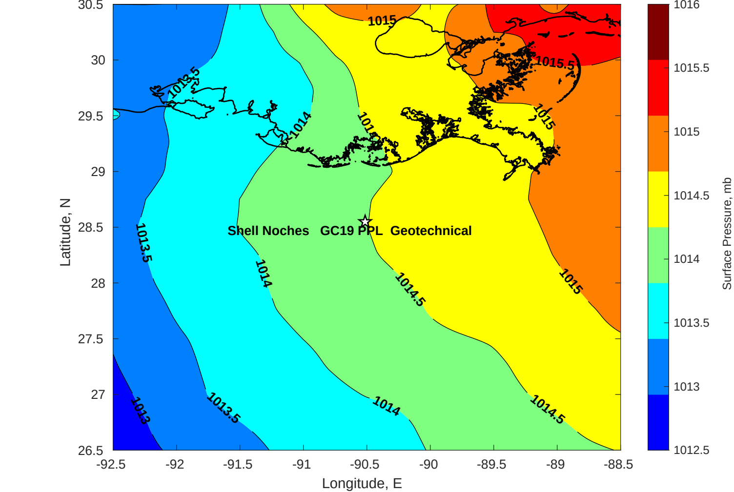
Surface Pressure (mb) for Shell Noches GC19 PPL Geotechnical at 02-May-2025 00:00:00
