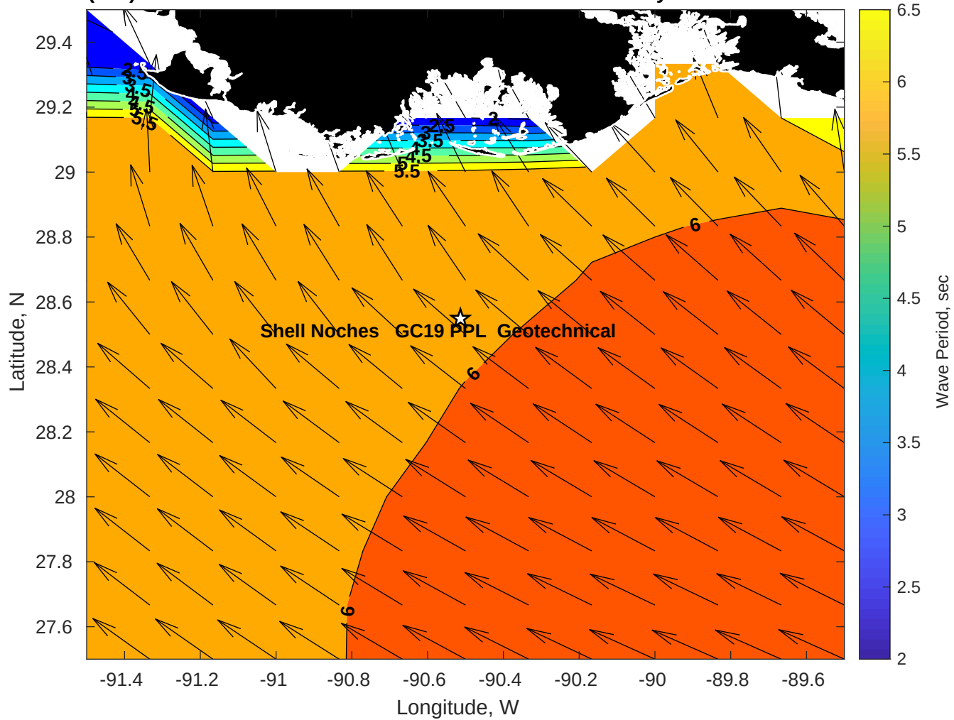
Wave Period (sec) for Shell Noches GC19 PPL Geotechnical at 02-May-2025 09:00:00
