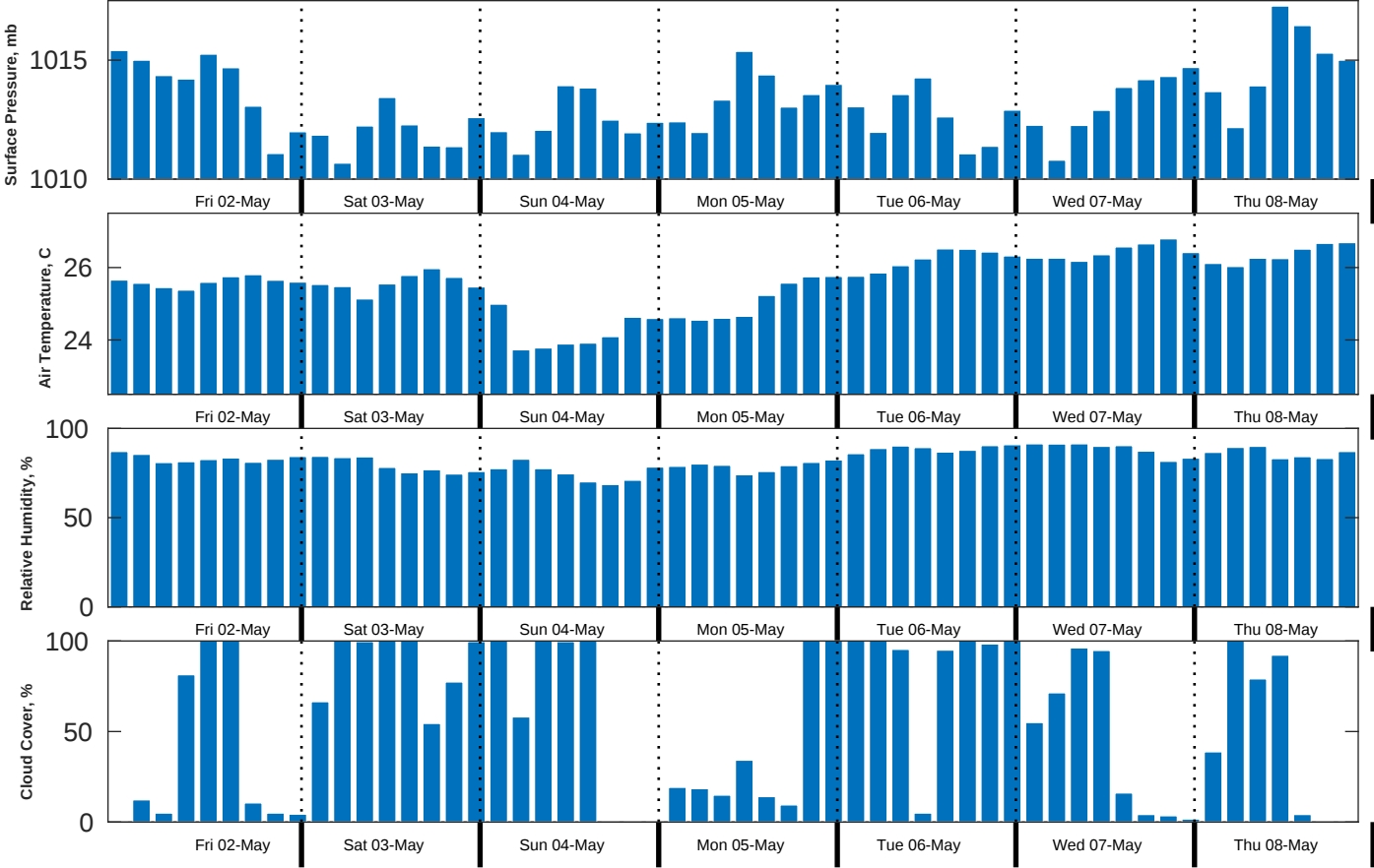
Met Forecast for Shell Noches GC19 PPL Geotechnical from 02-May-2025 00:00:00 to 09-May-2025 00:00:00
