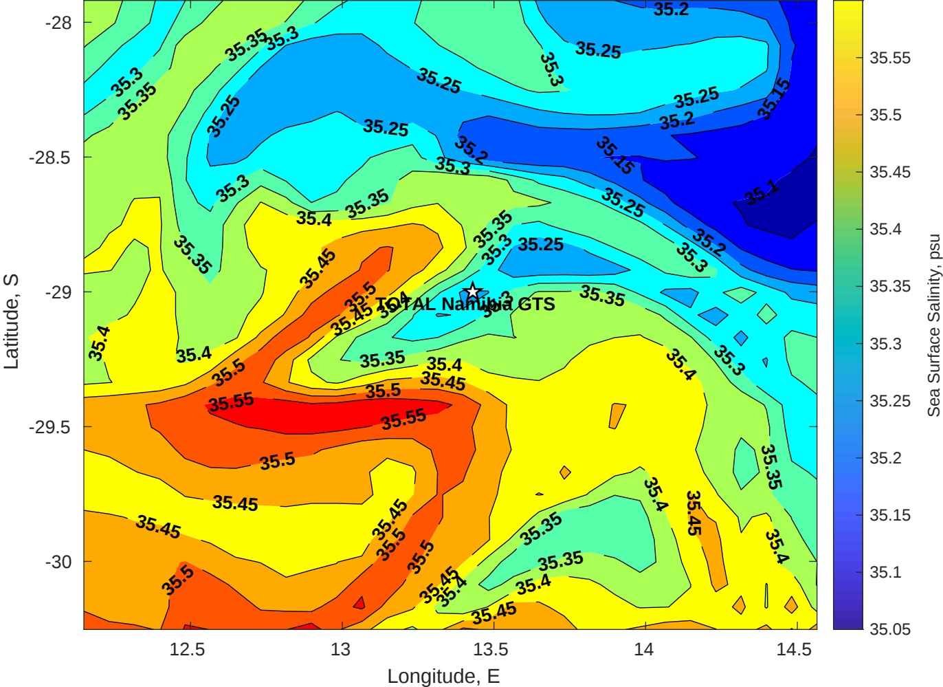
Surface Salinity for TOTAL Namibia GTS at 01-May-2025 00:00:00
