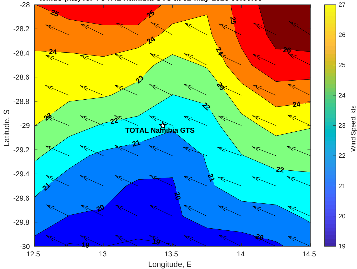
Winds (kts) for TOTAL Namibia GTS at 02-May-2025 09:00:00
