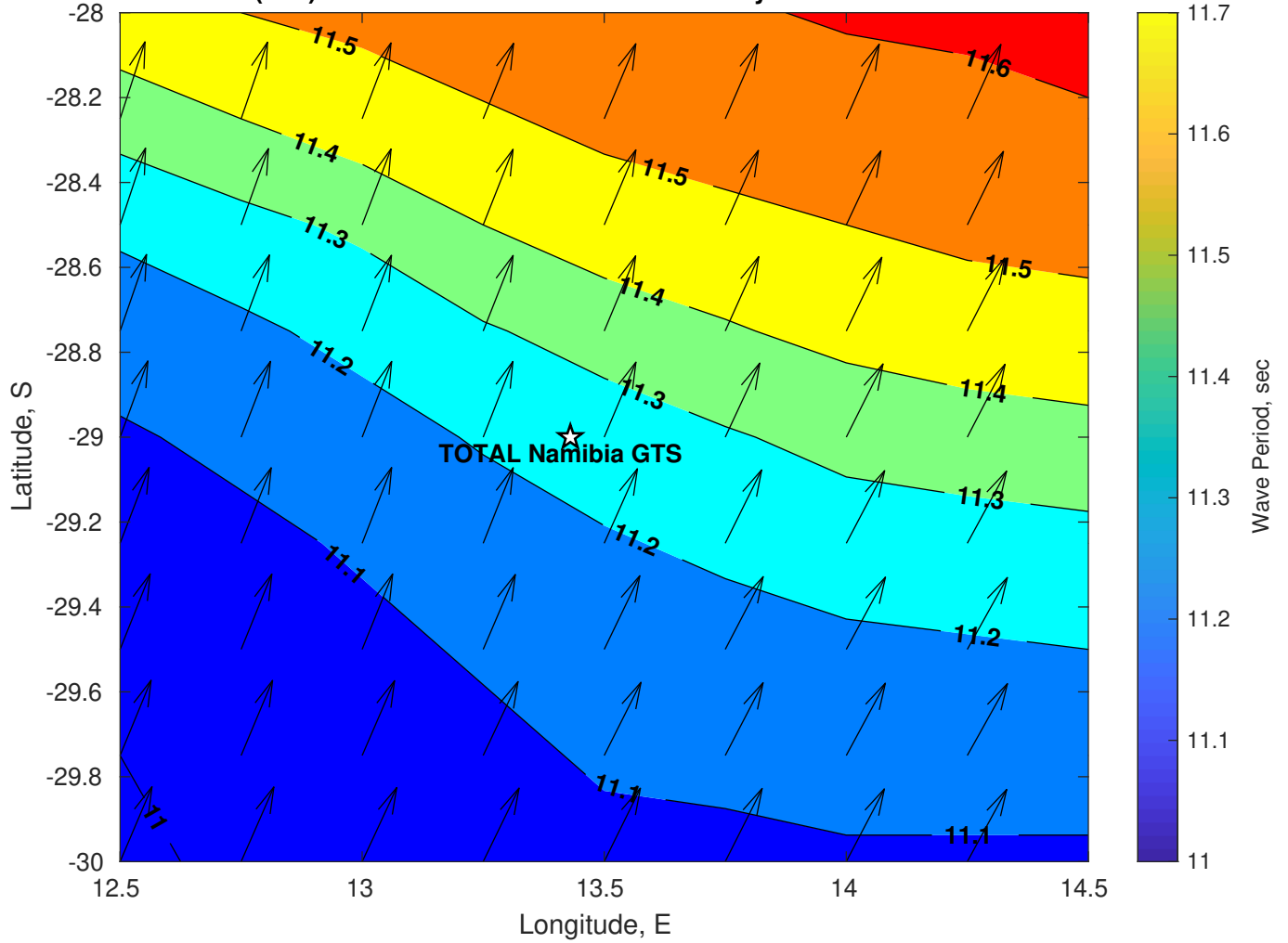
Wave Period (sec) for TOTAL Namibia GTS at 02-May-2025 09:00:00
