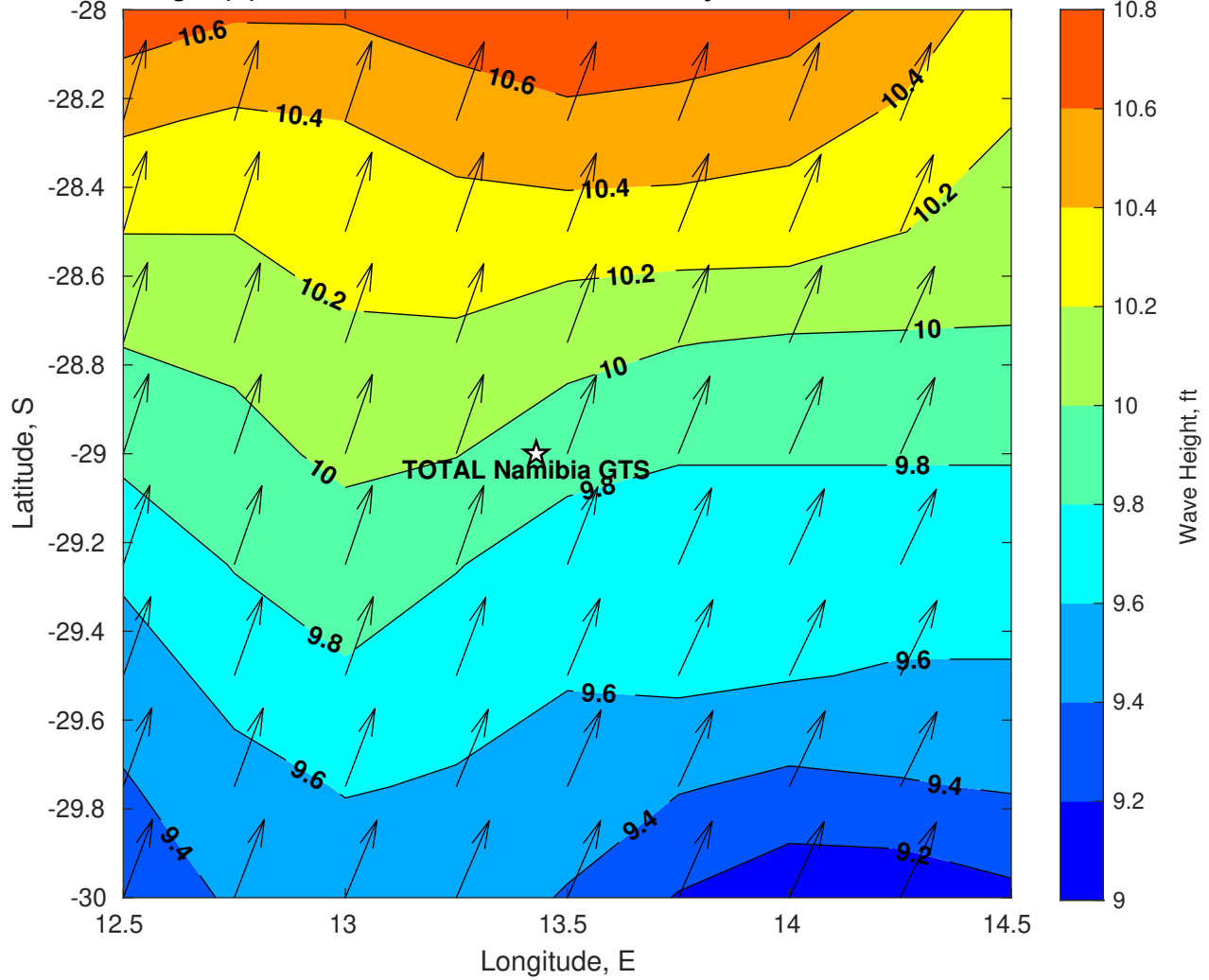
Wave Height (ft) for TOTAL Namibia GTS at 02-May-2025 09:00:00
