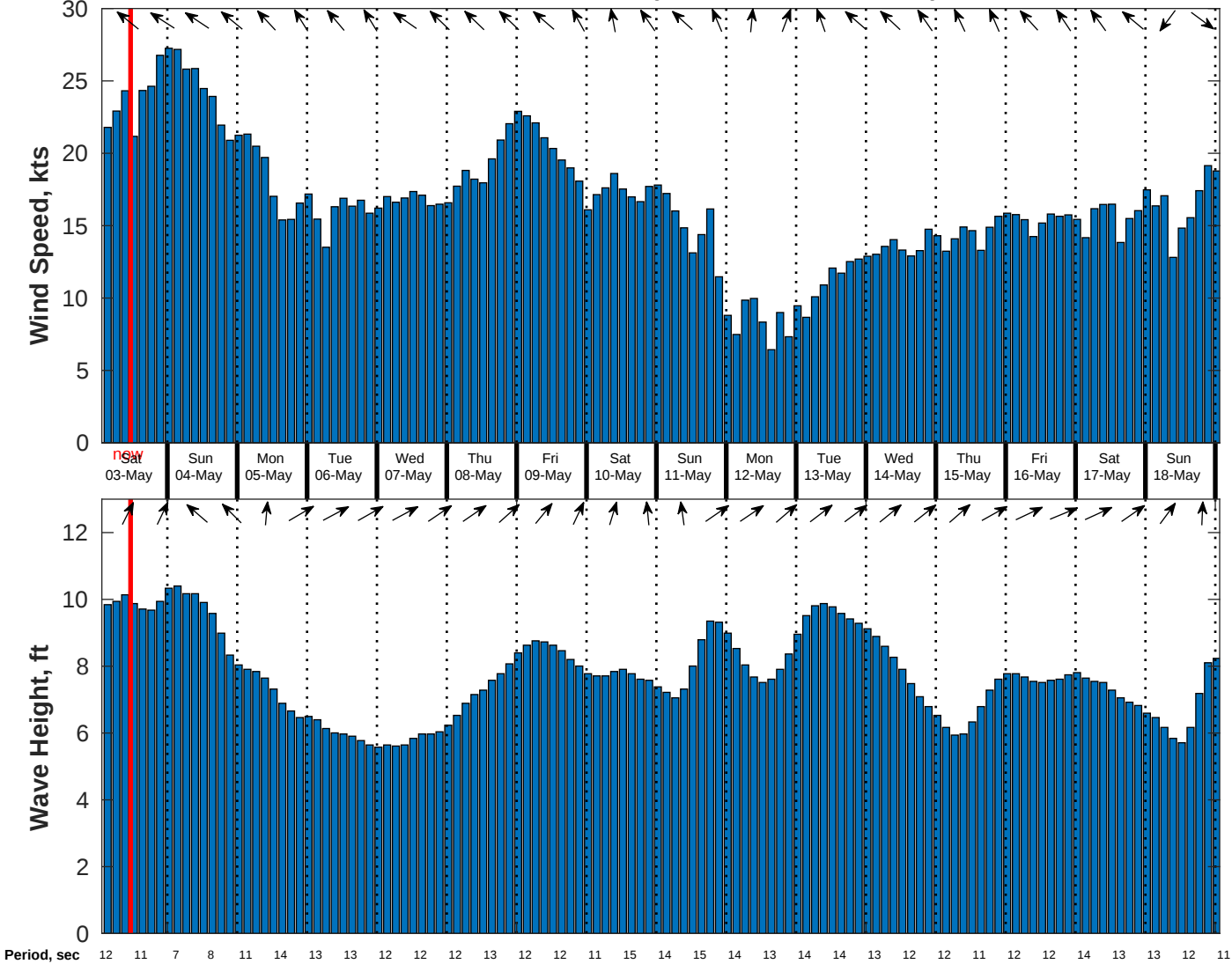
Wind & Wave Forecast for TOTAL Namibia GTS from 02-May-2025 02:00:00 to 18-May-2025 02:00:00
