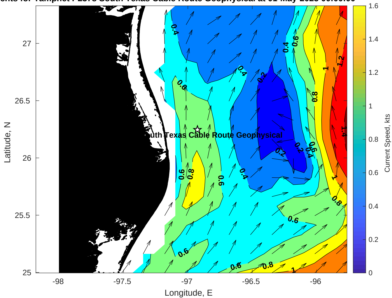
Surface Currents for Tampnet P2378 South Texas Cable Route Geophysical at 01-May-2025 00:00:00
