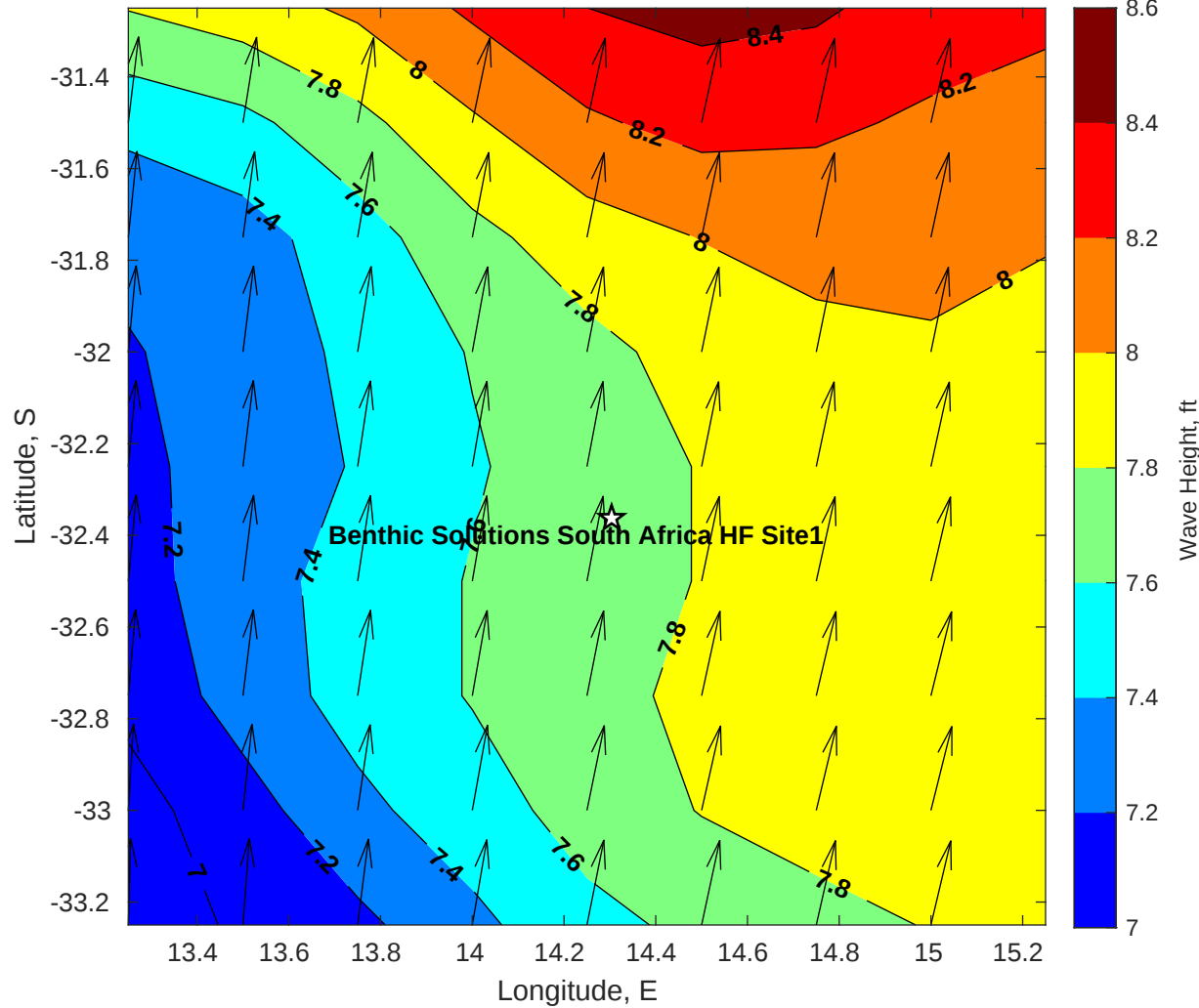
Wave Height (ft) for Benthic Solutions South Africa HF Site1 at 03-May-2025 09:00:00
