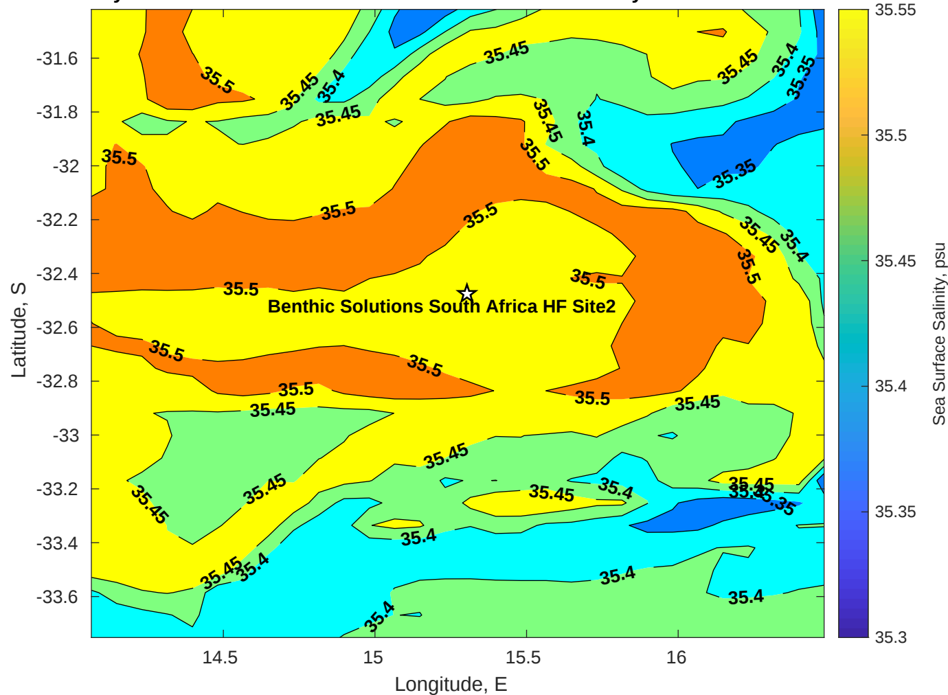
Surface Salinity for Benthic Solutions South Africa HF Site2 at 02-May-2025 00:00:00
