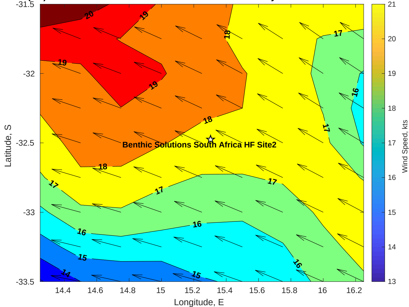
Winds (kts) for Benthic Solutions South Africa HF Site2 at 03-May-2025 09:00:00
