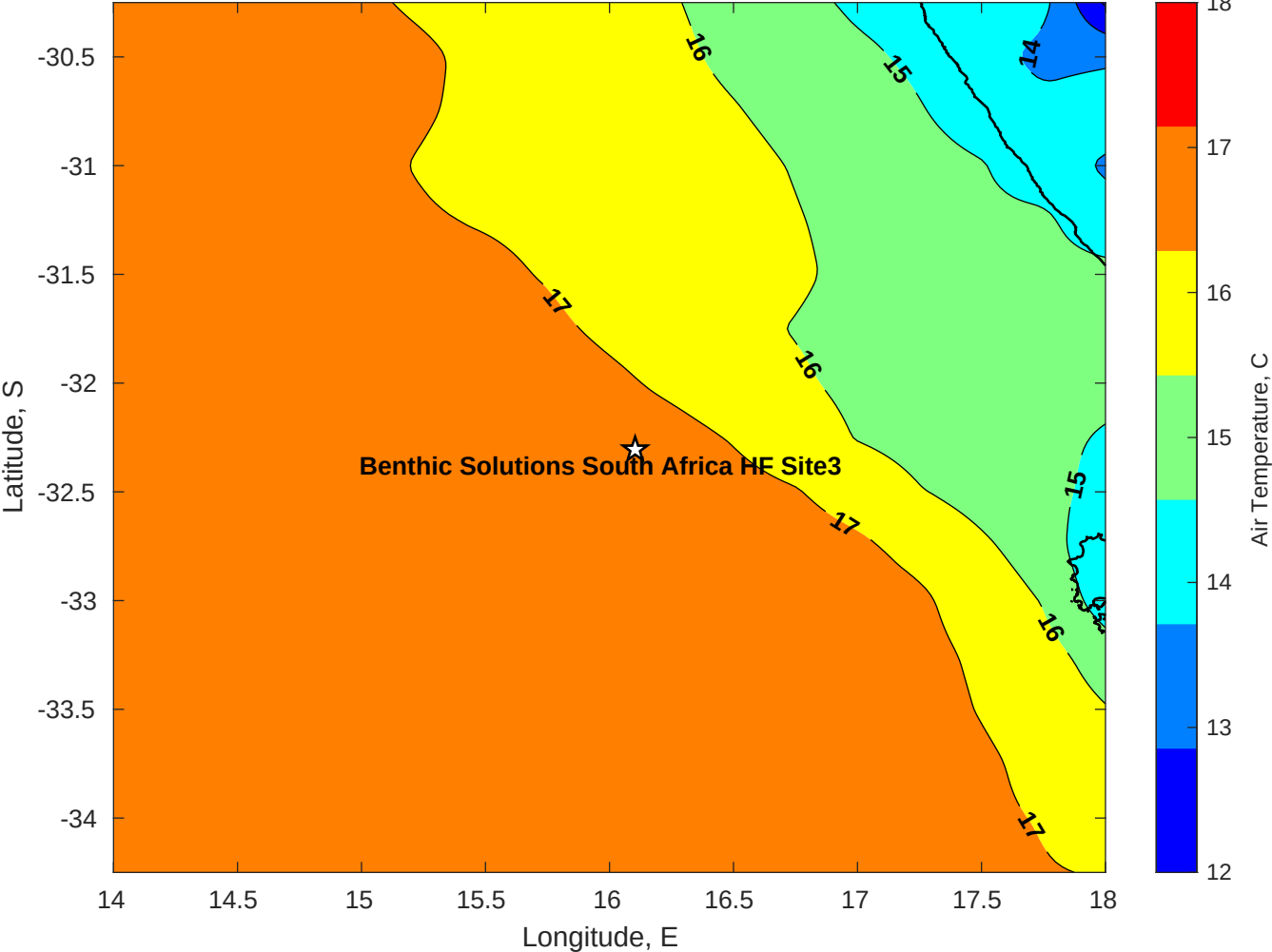
Air Temperature (C) for Benthic Solutions South Africa HF Site3 at 03-May-2025
