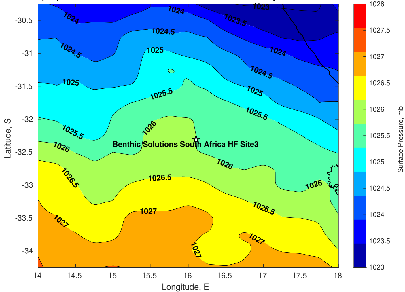
Surface Pressure (mb) for Benthic Solutions South Africa HF Site3 at 03-May-2025 00:00:00
