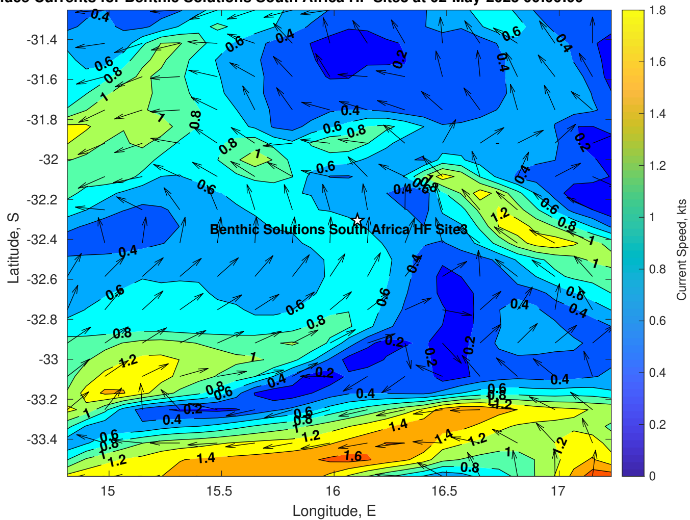
Surface Currents for Benthic Solutions South Africa HF Site3 at 02-May-2025 00:00:00
