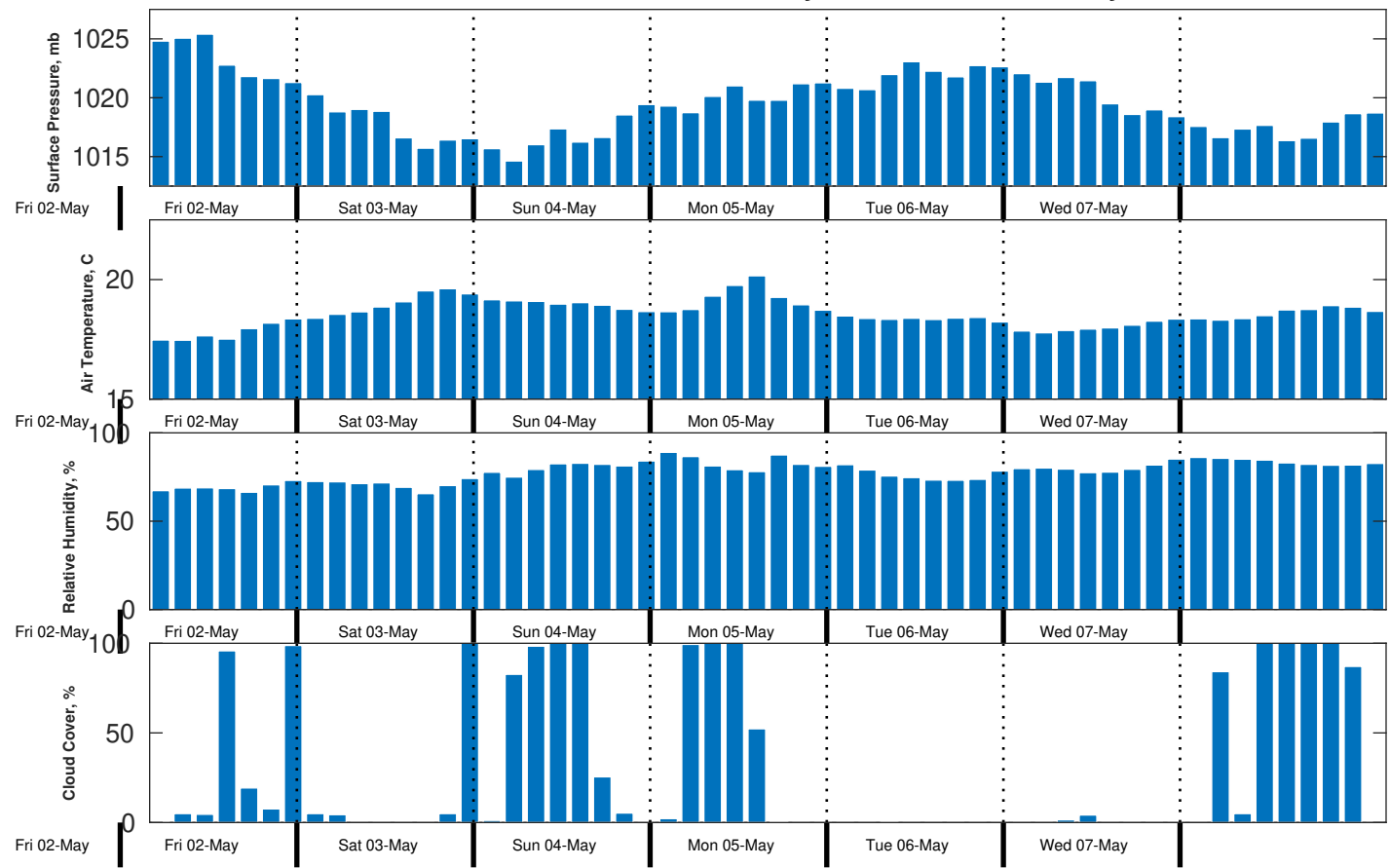
Met Forecast for Benthic Solutions South Africa HF Site3 from 03-May-2025 00:00:00 to 10-May-2025 00:00:00
