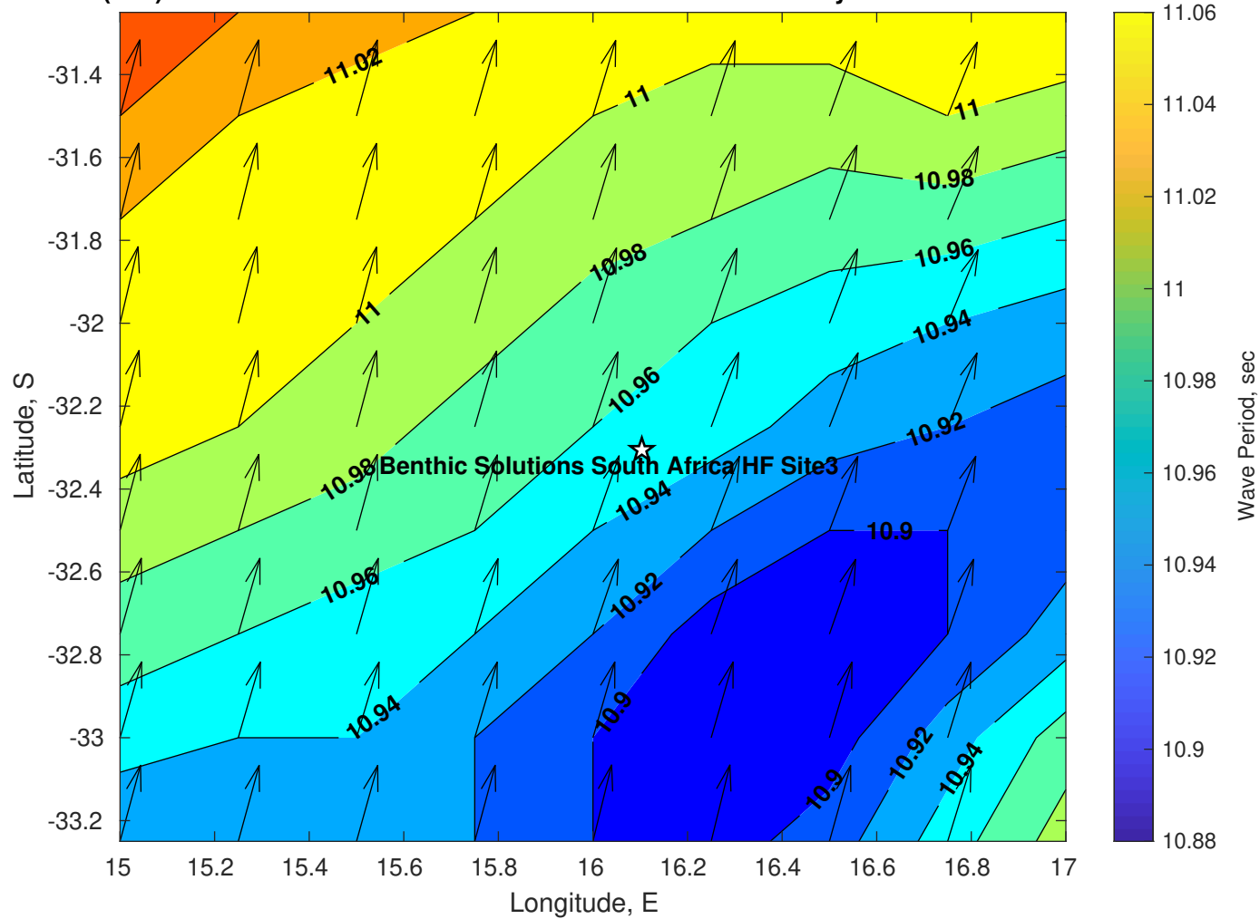
Wave Period (sec) for Benthic Solutions South Africa HF Site3 at 03-May-2025 09:00:00
