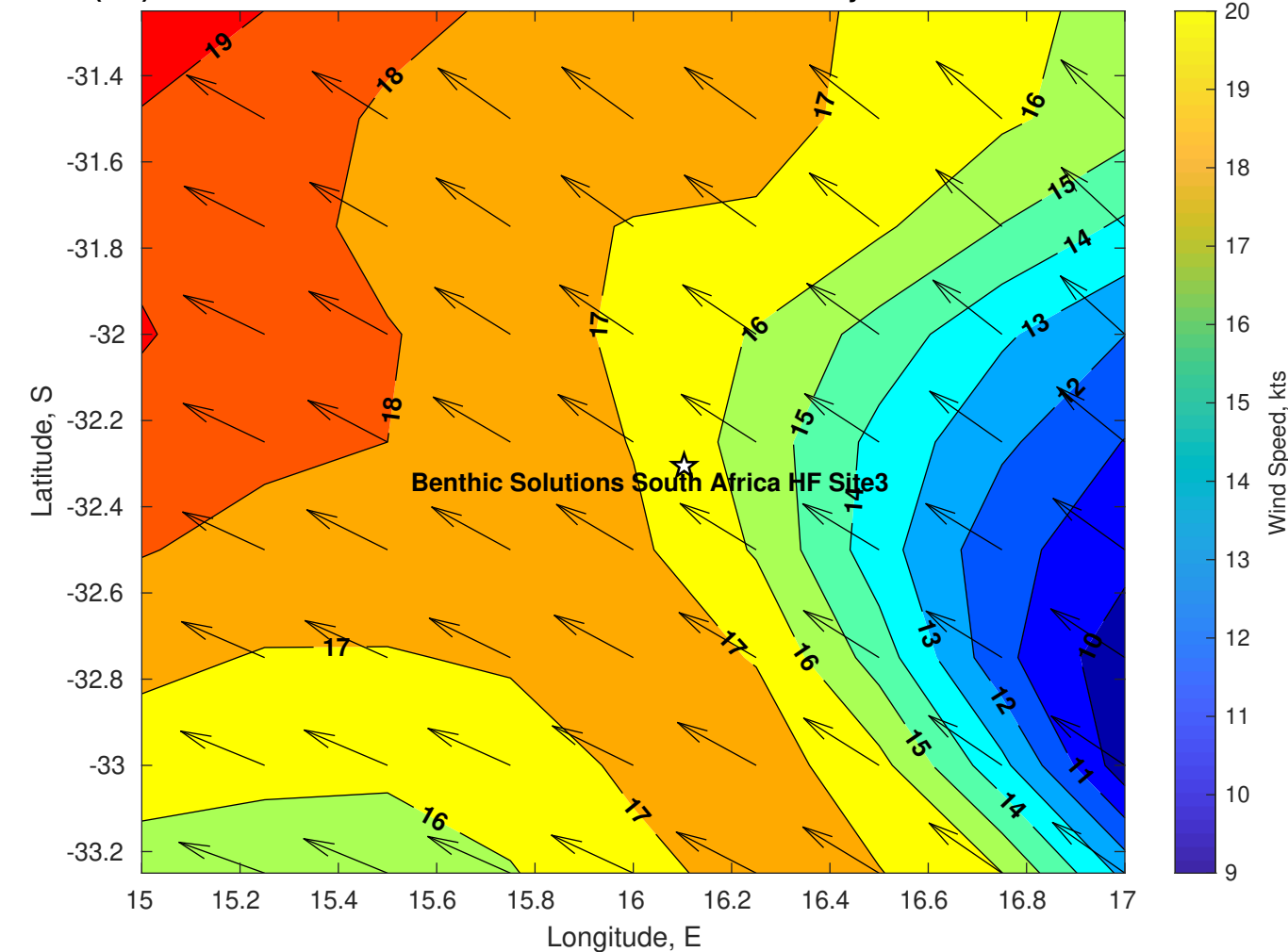
Winds (kts) for Benthic Solutions South Africa HF Site3 at 03-May-2025 09:00:00
