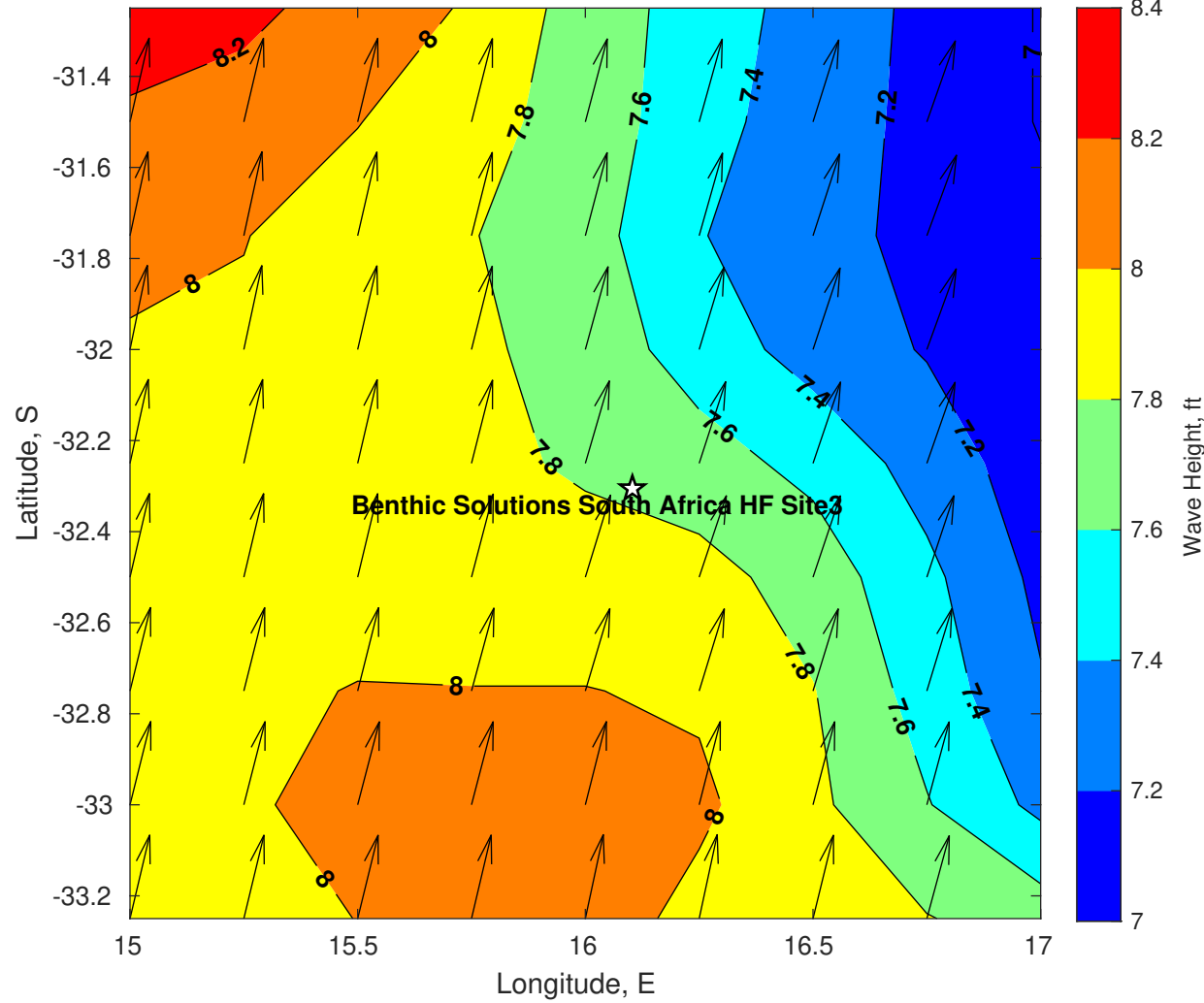
Wave Height (ft) for Benthic Solutions South Africa HF Site3 at 03-May-2025 09:00:00
