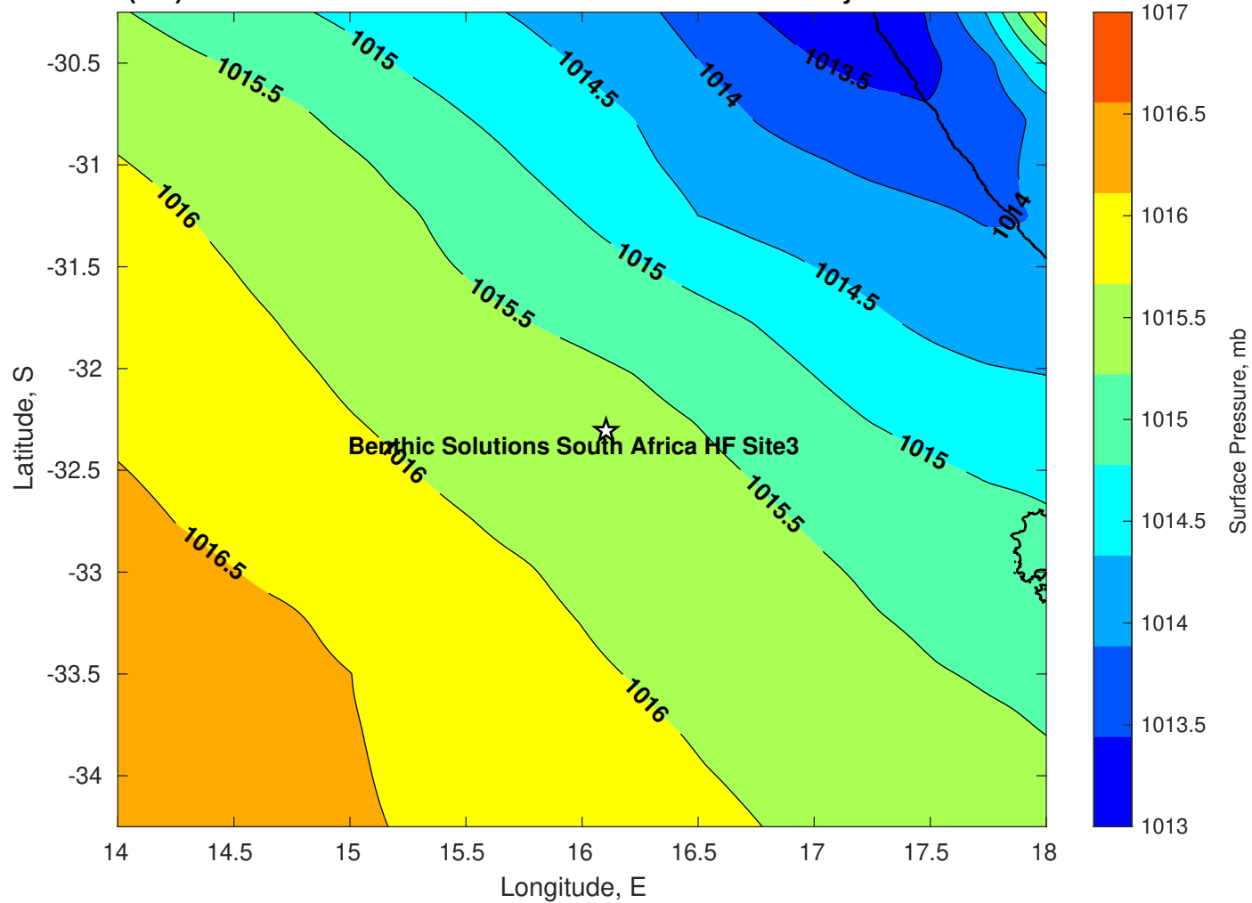
Surface Pressure (mb) for Benthic Solutions South Africa HF Site3 at 05-May-2025 00:00:00
