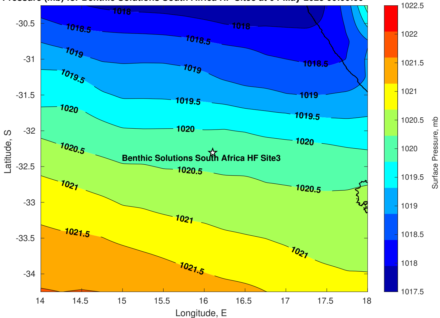
Surface Pressure (mb) for Benthic Solutions South Africa HF Site3 at 04-May-2025 00:00:00
