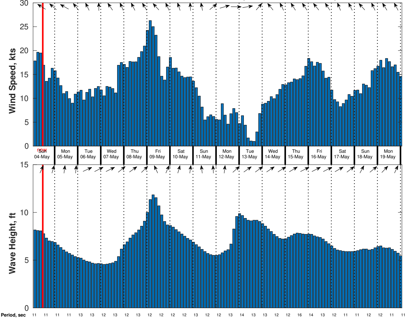
Wind & Wave Forecast for Benthic Solutions South Africa HF Site3 from 03-May-2025 02:00:00 to 19-May-2025 02:00:00
