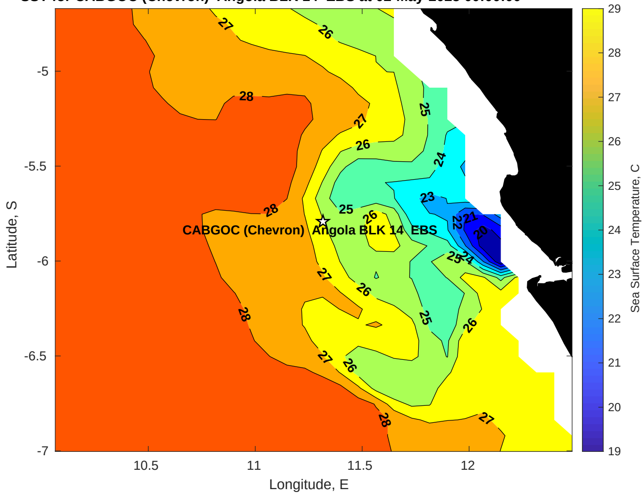
SST for CABGOC (Chevron) Angola BLK 14 EBS at 02-May-2025 00:00:00
