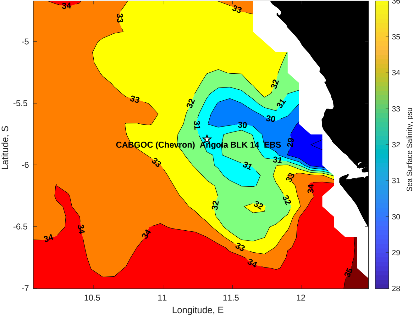
Surface Salinity for CABGOC (Chevron) Angola BLK 14 EBS at 02-May-2025 00:00:00
