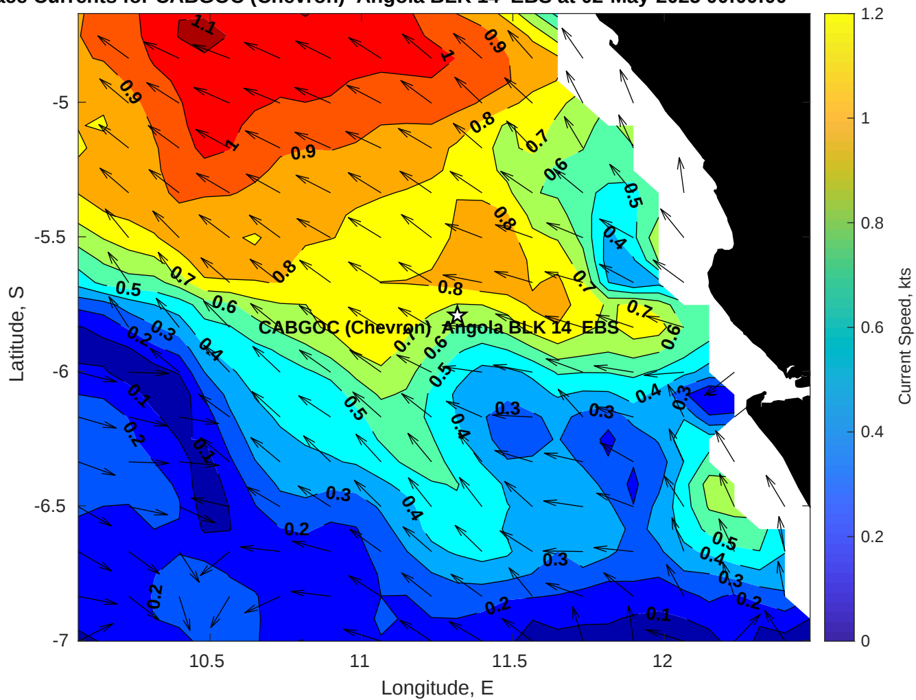
Surface Currents for CABGOC (Chevron) Angola BLK 14 EBS at 02-May-2025 00:00:00
