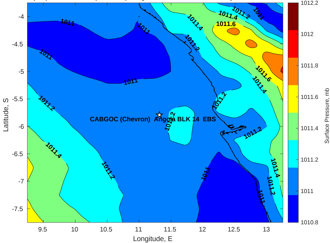
Surface Pressure (mb) for CABGOC (Chevron) Angola BLK 14 EBS at 03-May-2025 00:00:00
