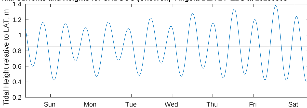
Tidal Currents and Heights for CABGOC (Chevron) Angola BLK 14 EBS at 20250503
