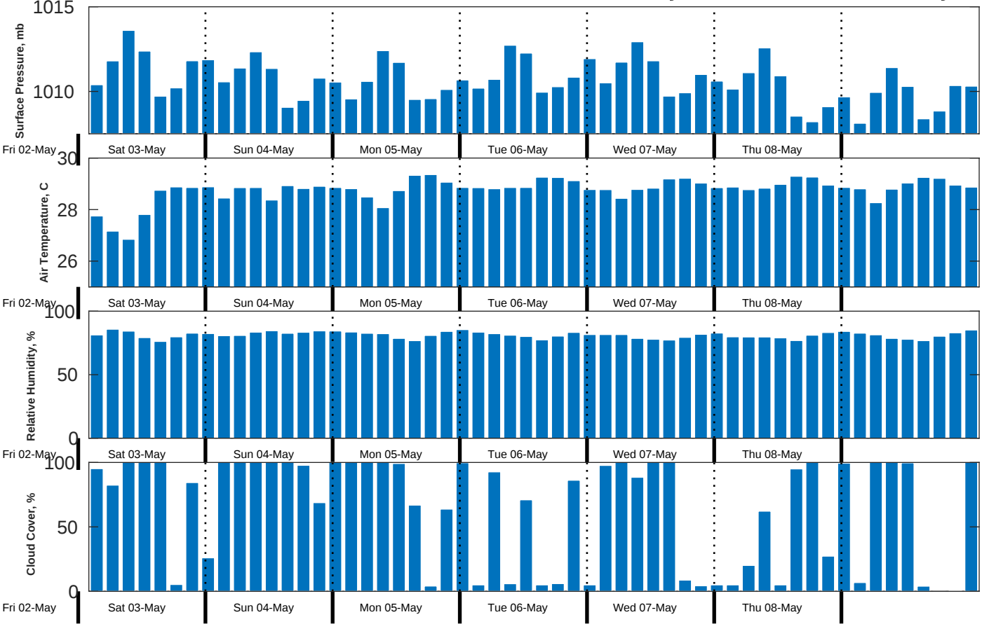
Met Forecast for CSA (ONHYM) PPL EBS - Cote d'Ivoire from 03-May-2025 00:00:00 to 10-May-2025 00:00:00
