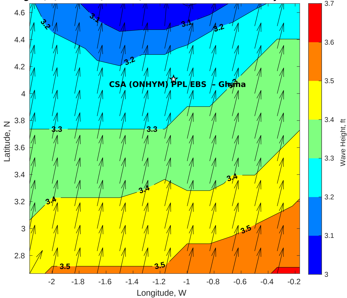
Wave Height (ft) for CSA (ONHYM) PPL EBS - Ghana at 03-May-2025 09:00:00
