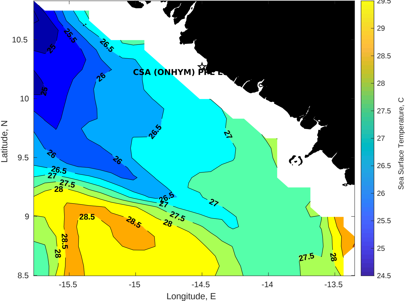
SST for CSA (ONHYM) PPL EBS - Guinea at 02-May-2025 00:00:00
