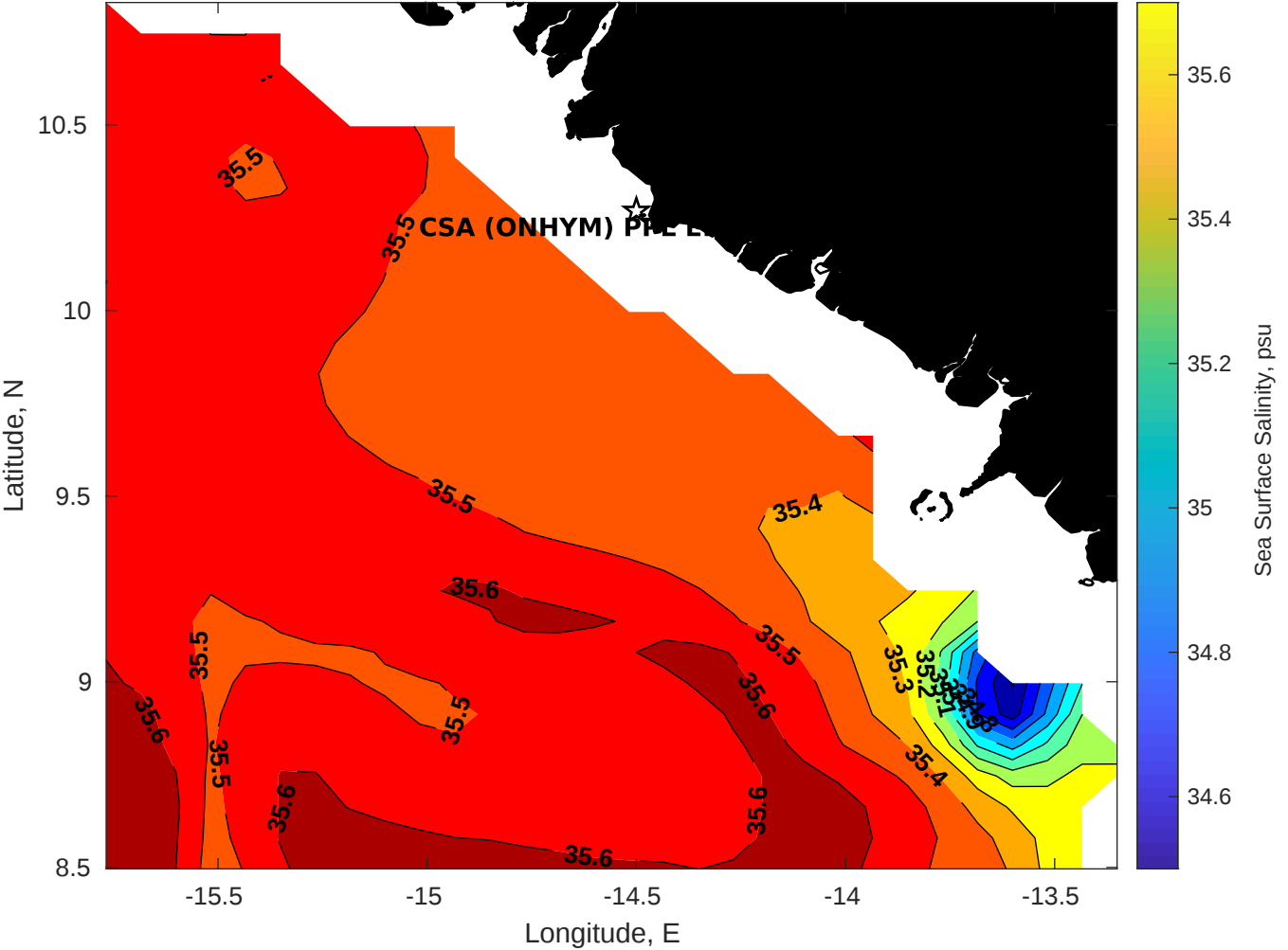
Surface Salinity for CSA (ONHYM) PPL EBS - Guinea at 02-May-2025 00:00:00
