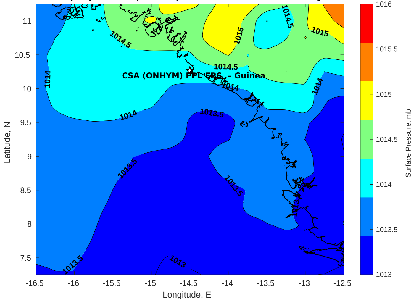
Surface Pressure (mb) for CSA (ONHYM) PPL EBS - Guinea at 04-May-2025 00:00:00
