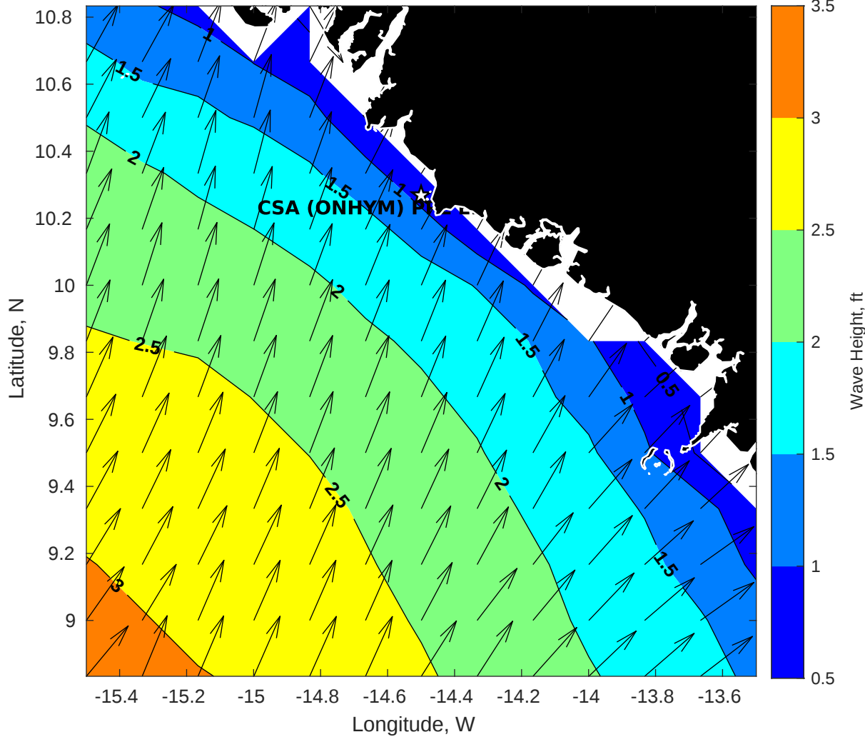
Wave Height (ft) for CSA (ONHYM) PPL EBS - Guinea at 03-May-2025 09:00:00
