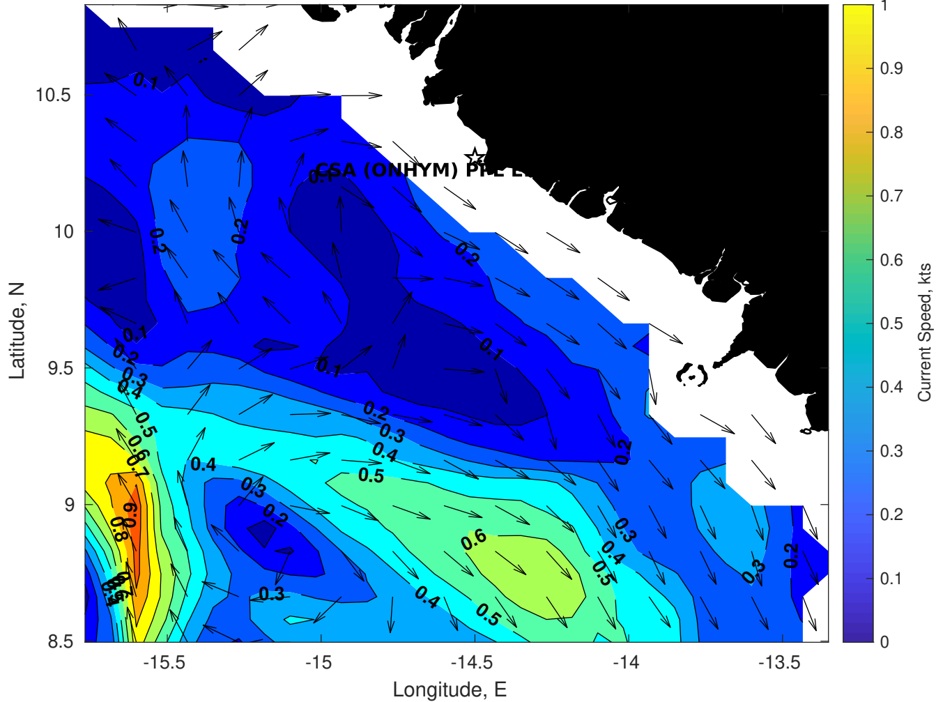
Surface Currents for CSA (ONHYM) PPL EBS - Guinea at 02-May-2025 00:00:00
