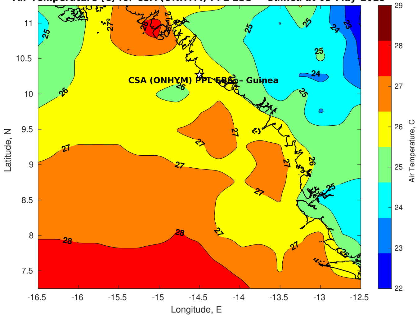
Air Temperature (C) for CSA (ONHYM) PPL EBS - Guinea at 03-May-2025
