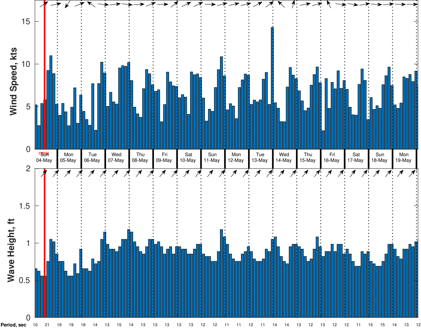
Wind & Wave Forecast for CSA (ONHYM) PPL EBS - Guinea from 03-May-2025 01:00:00 to 19-May-2025 01:00:00
