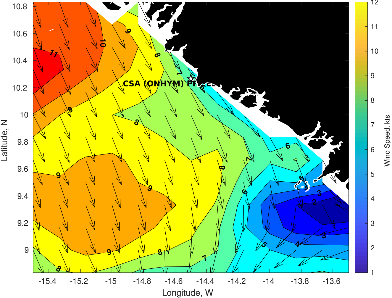
Winds (kts) for CSA (ONHYM) PPL EBS - Guinea at 03-May-2025 09:00:00
