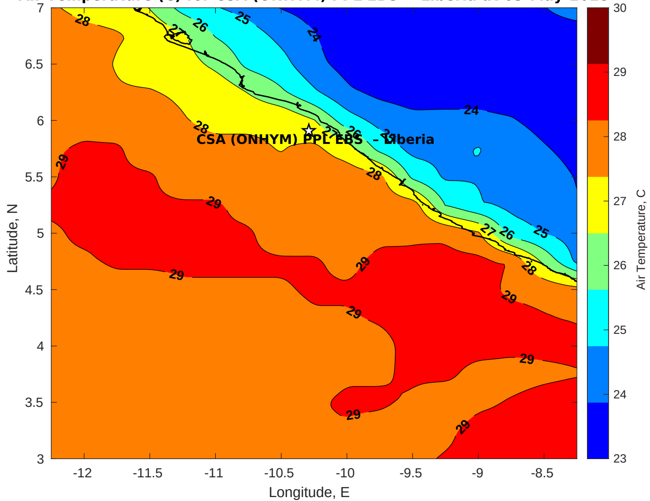
Air Temperature (C) for CSA (ONHYM) PPL EBS - Liberia at 03-May-2025
