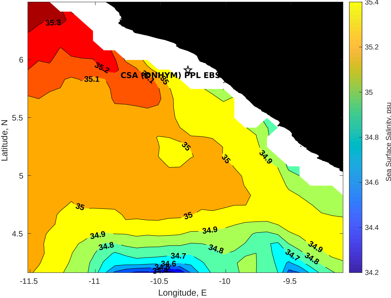
Surface Salinity for CSA (ONHYM) PPL EBS - Liberia at 02-May-2025 00:00:00
